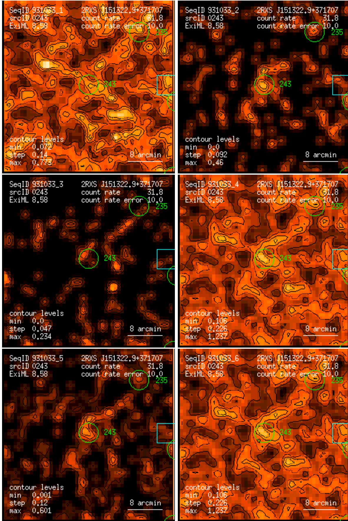
Figure 243: RASS 931033: detection 0243: band rate images, Gaussian filter: (1) PSPC channels 11 – 41, (2) 52 – 90, (3) 91 – 201, (4) 11 – 235, (5) 52 – 201, (6) 11 – 201. Broad band rates in counts/ks. Band rate contour levels in counts/ks/arcmin 2 .
