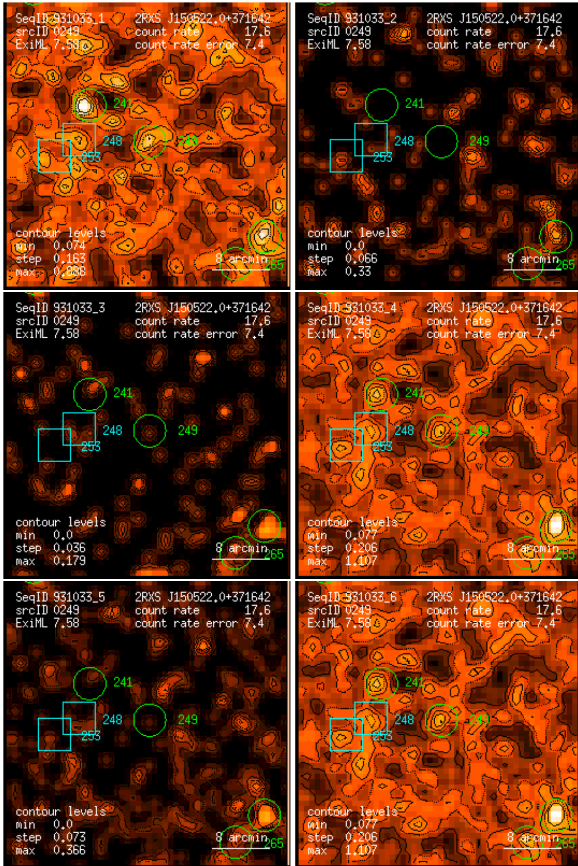
Figure 249: RASS 931033: detection 0249: band rate images, Gaussian filter: (1) PSPC channels 11 – 41, (2) 52 – 90, (3) 91 – 201, (4) 11 – 235, (5) 52 – 201, (6) 11 – 201. Broad band rates in counts/ks. Band rate contour levels in counts/ks/arcmin 2 .
