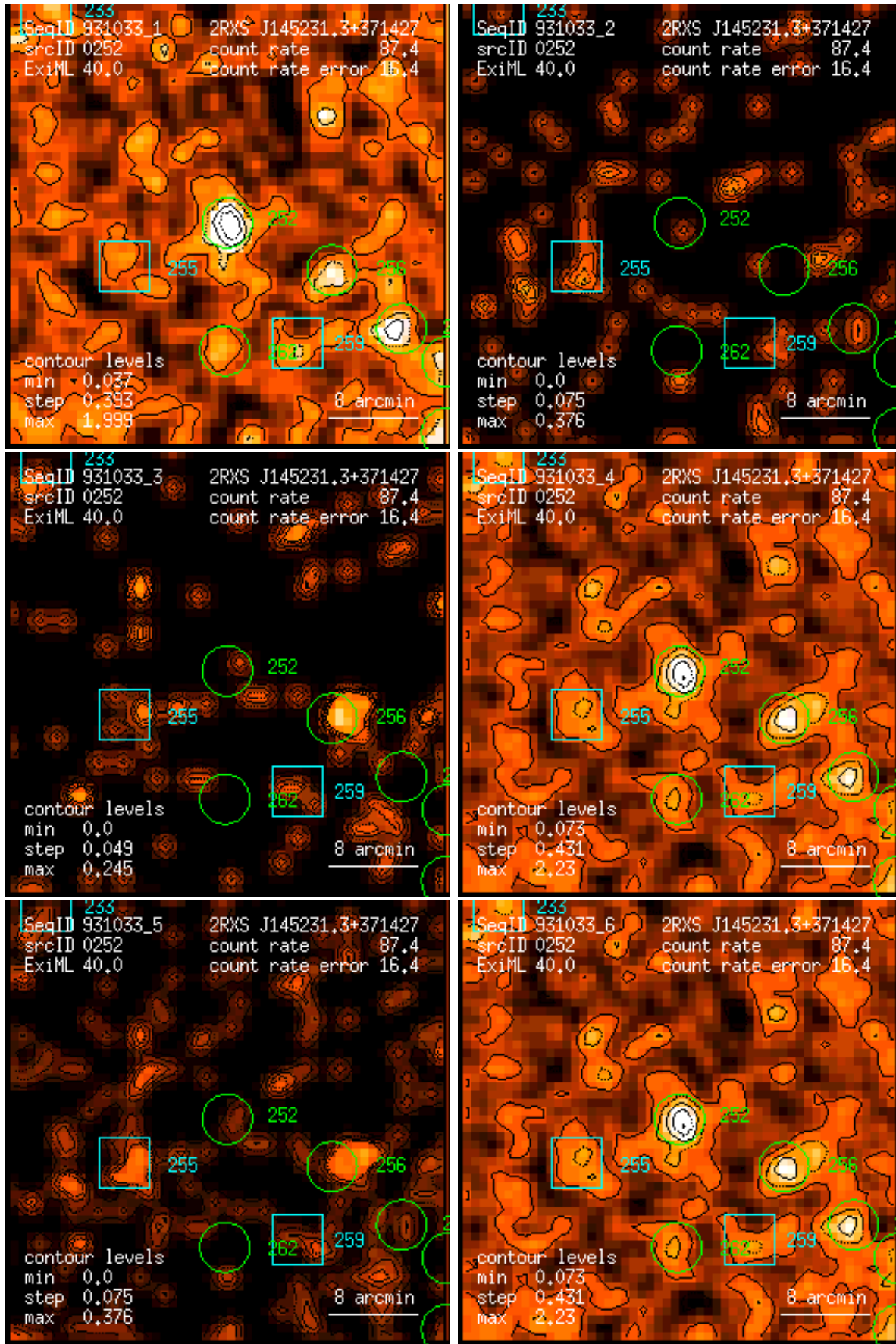
Figure 252: RASS 931033: detection 0252: band rate images, Gaussian filter: (1) PSPC channels 11 – 41, (2) 52 – 90, (3) 91 – 201, (4) 11 – 235, (5) 52 – 201, (6) 11 – 201. Broad band rates in counts/ks. Band rate contour levels in counts/ks/arcmin 2 .
