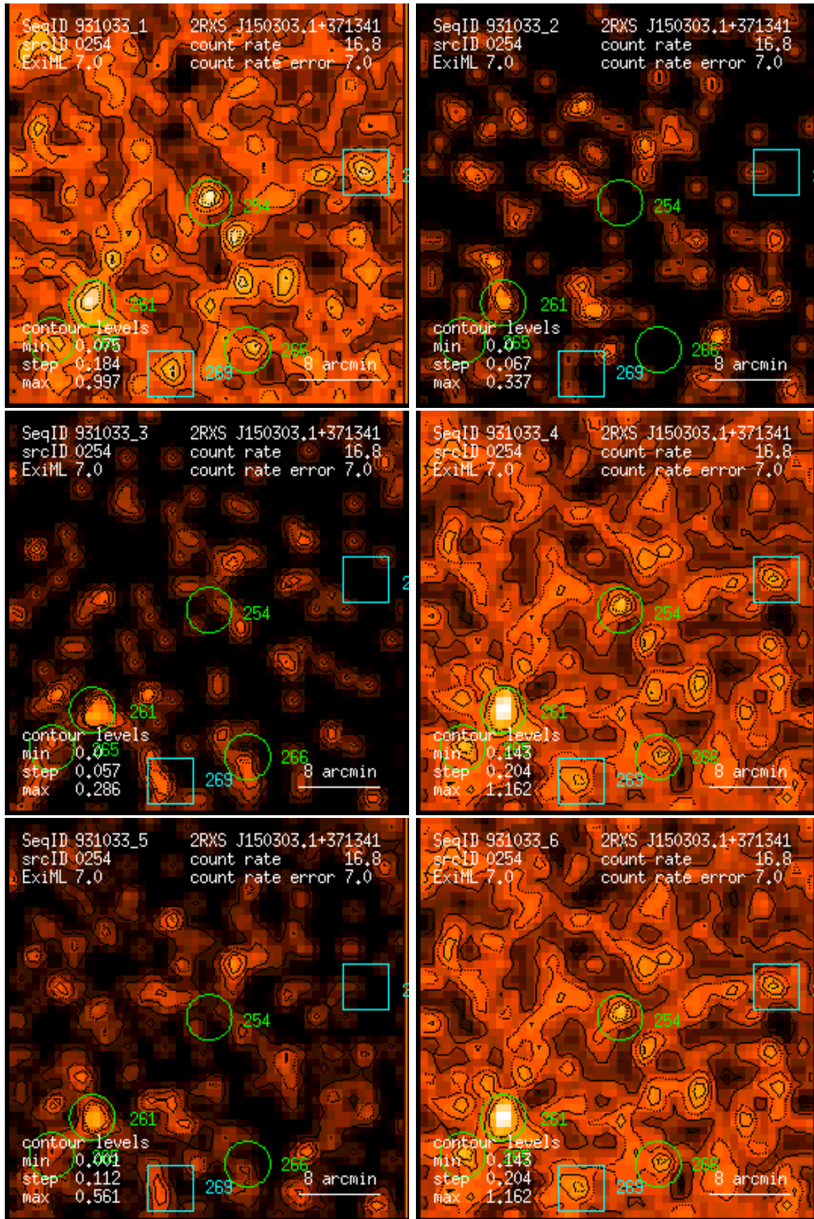
Figure 254: RASS 931033: detection 0254: band rate images, Gaussian filter: (1) PSPC channels 11 – 41, (2) 52 – 90, (3) 91 – 201, (4) 11 – 235, (5) 52 – 201, (6) 11 – 201. Broad band rates in counts/ks. Band rate contour levels in counts/ks/arcmin 2 .
