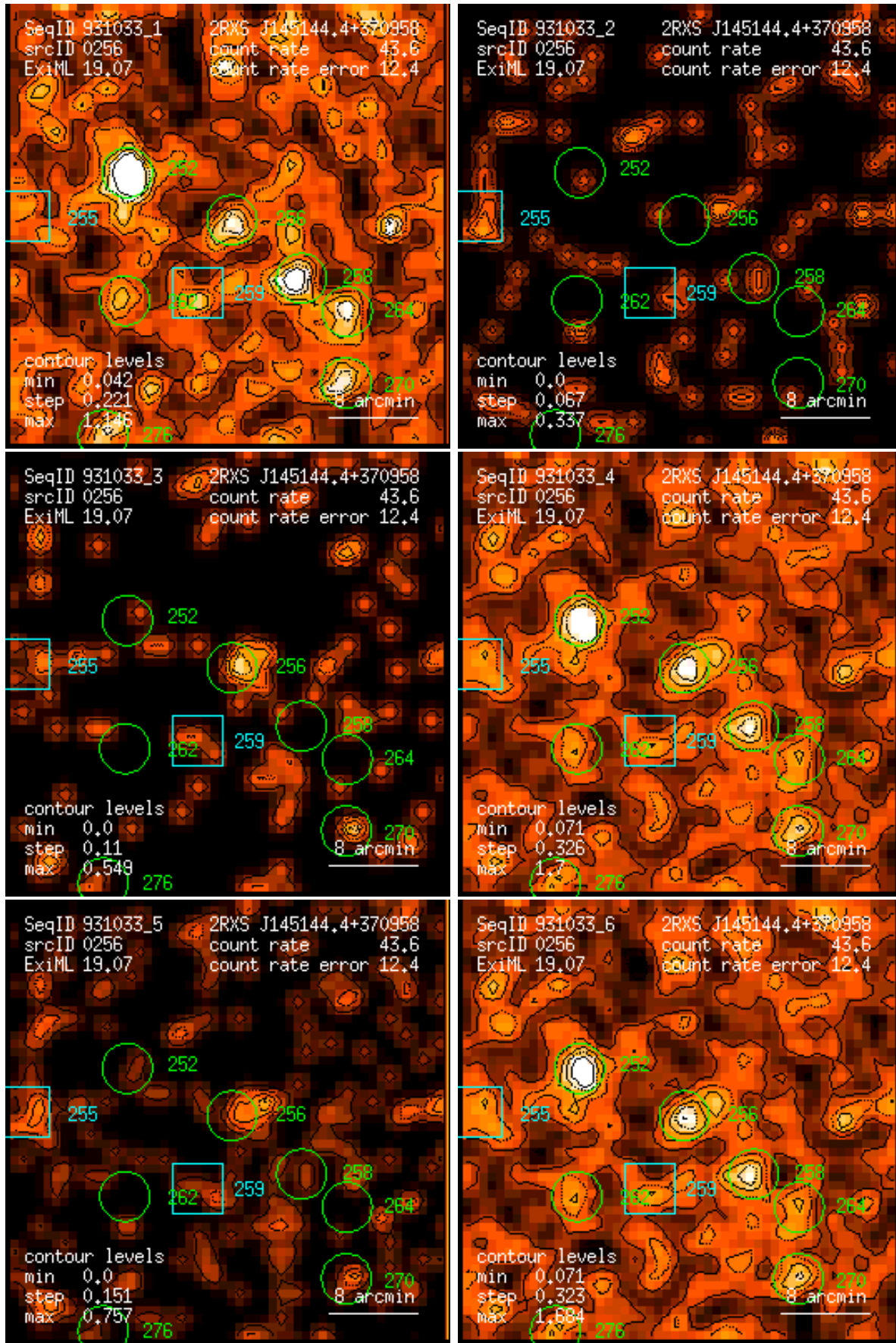
Figure 256: RASS 931033: detection 0256: band rate images, Gaussian filter: (1) PSPC channels 11 – 41, (2) 52 – 90, (3) 91 – 201, (4) 11 – 235, (5) 52 – 201, (6) 11 – 201. Broad band rates in counts/ks. Band rate contour levels in counts/ks/arcmin 2 .
