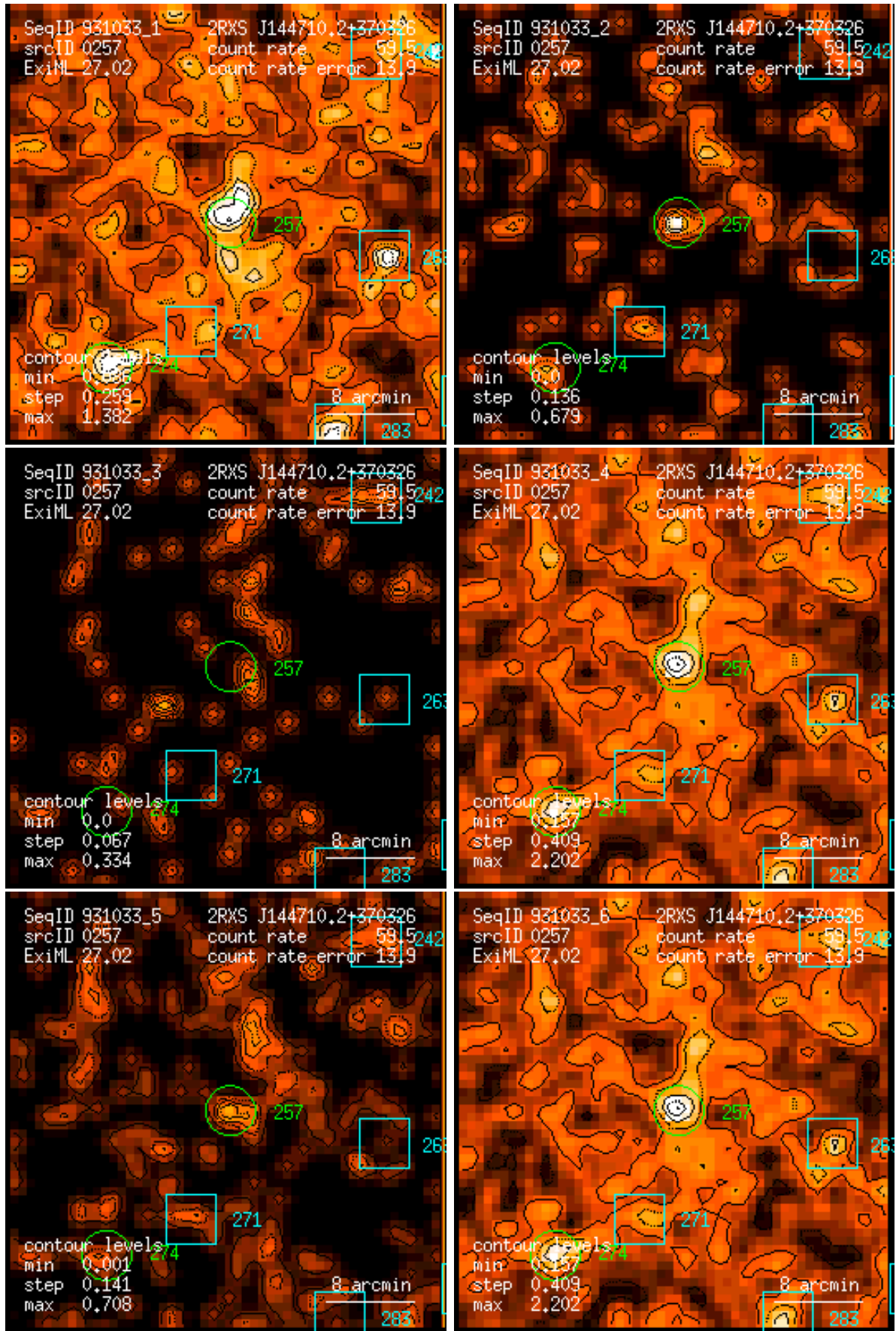
Figure 257: RASS 931033: detection 0257: band rate images, Gaussian filter: (1) PSPC channels 11 – 41, (2) 52 – 90, (3) 91 – 201, (4) 11 – 235, (5) 52 – 201, (6) 11 – 201. Broad band rates in counts/ks. Band rate contour levels in counts/ks/arcmin 2 .
