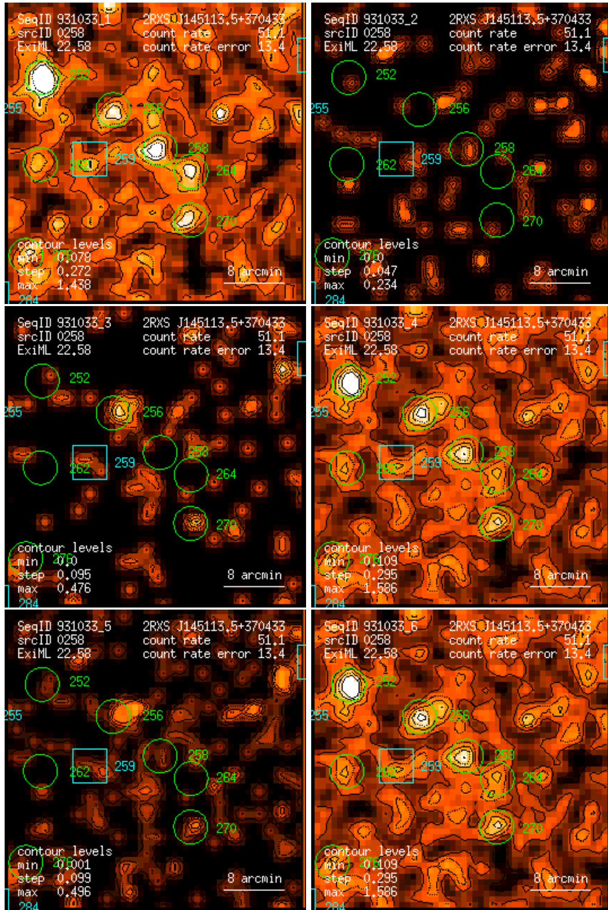
Figure 258: RASS 931033: detection 0258: band rate images, Gaussian filter: (1) PSPC channels 11 – 41, (2) 52 – 90, (3) 91 – 201, (4) 11 – 235, (5) 52 – 201, (6) 11 – 201. Broad band rates in counts/ks. Band rate contour levels in counts/ks/arcmin 2 .
