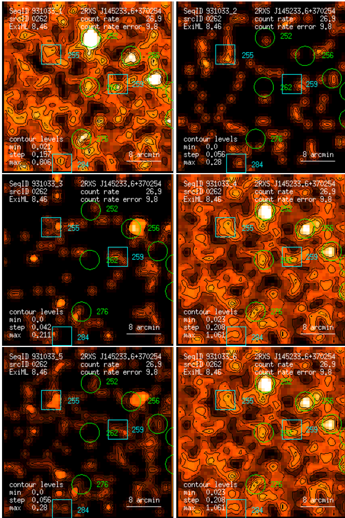
Figure 262: RASS 931033: detection 0262: band rate images, Gaussian filter: (1) PSPC channels 11 – 41, (2) 52 – 90, (3) 91 – 201, (4) 11 – 235, (5) 52 – 201, (6) 11 – 201. Broad band rates in counts/ks. Band rate contour levels in counts/ks/arcmin 2 .
