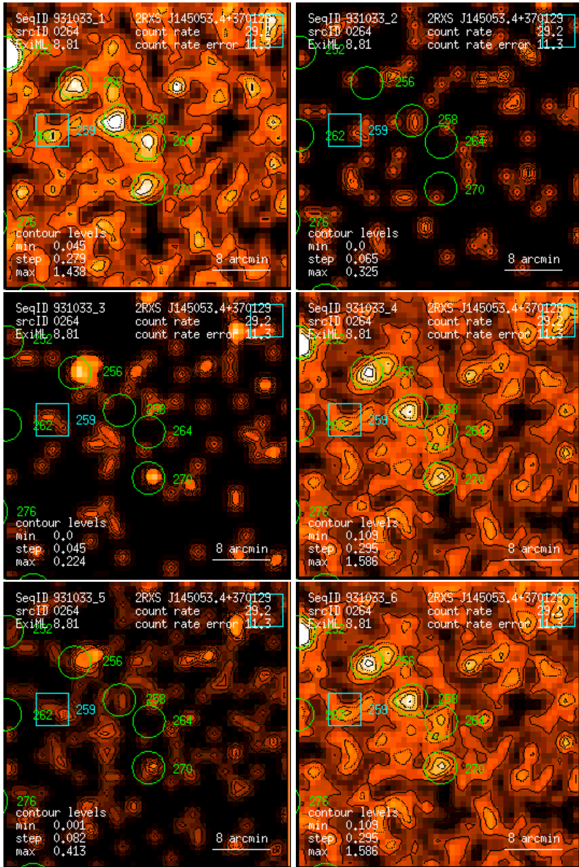
Figure 264: RASS 931033: detection 0264: band rate images, Gaussian filter: (1) PSPC channels 11 – 41, (2) 52 – 90, (3) 91 – 201, (4) 11 – 235, (5) 52 – 201, (6) 11 – 201. Broad band rates in counts/ks. Band rate contour levels in counts/ks/arcmin 2 .
