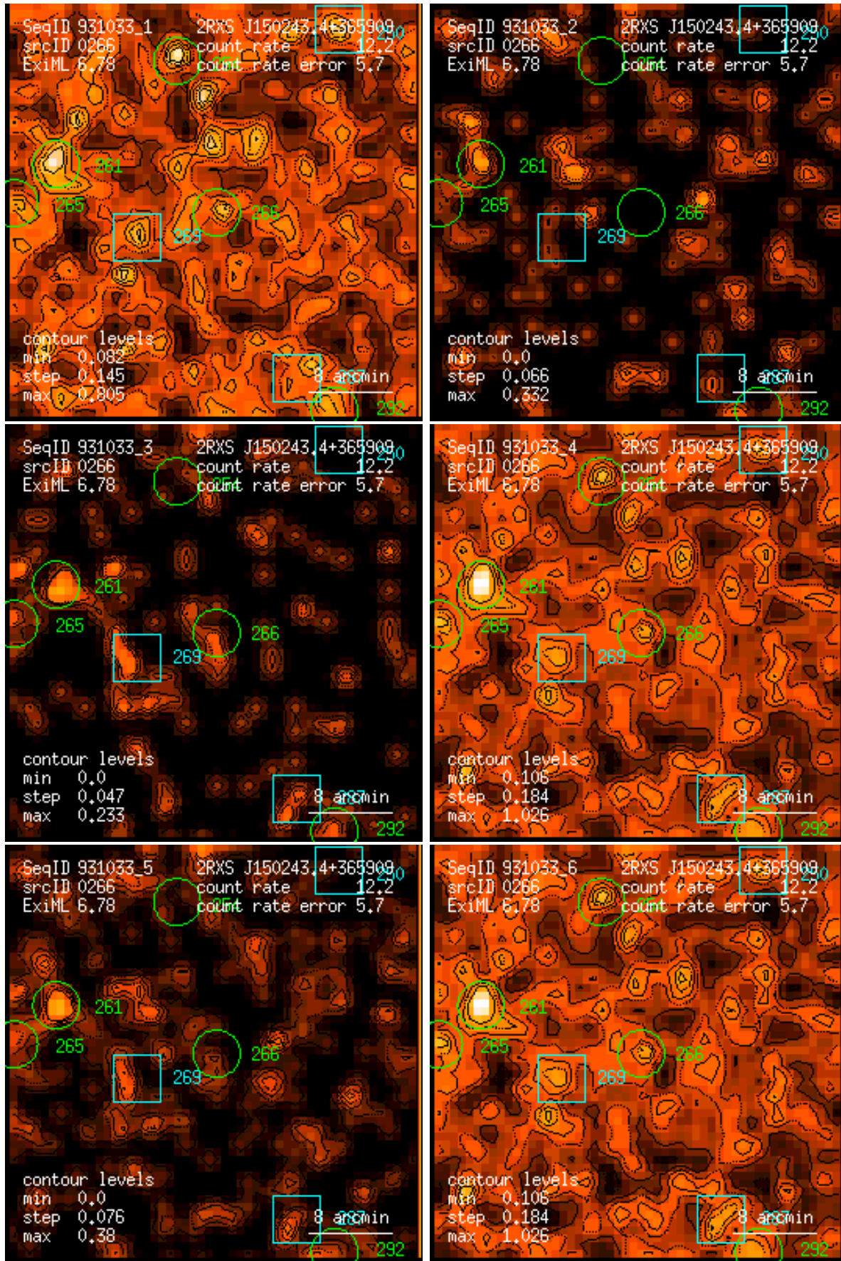
Figure 266: RASS 931033: detection 0266: band rate images, Gaussian filter: (1) PSPC channels 11 – 41, (2) 52 – 90, (3) 91 – 201, (4) 11 – 235, (5) 52 – 201, (6) 11 – 201. Broad band rates in counts/ks. Band rate contour levels in counts/ks/arcmin 2 .
