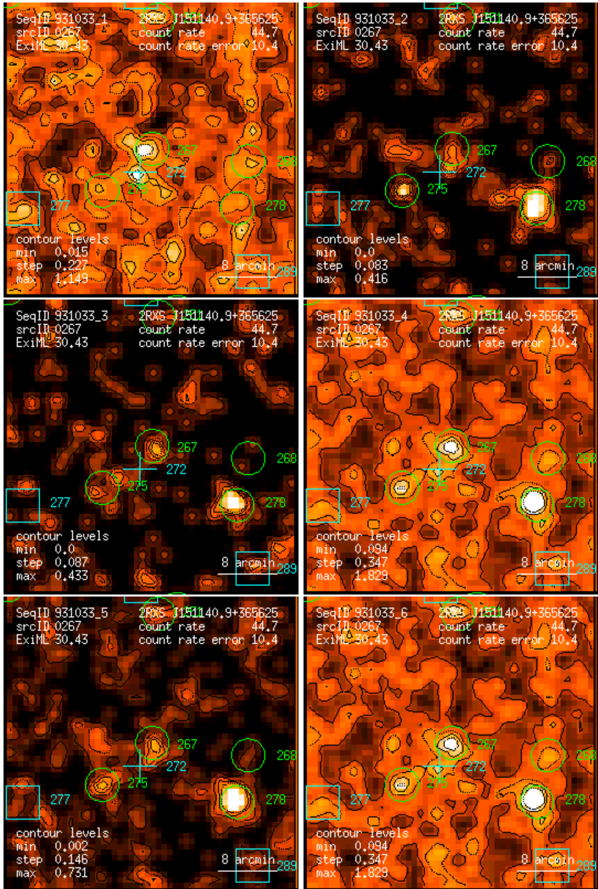
Figure 267: RASS 931033: detection 0267: band rate images, Gaussian filter: (1) PSPC channels 11 – 41, (2) 52 – 90, (3) 91 – 201, (4) 11 – 235, (5) 52 – 201, (6) 11 – 201. Broad band rates in counts/ks. Band rate contour levels in counts/ks/arcmin 2 .
