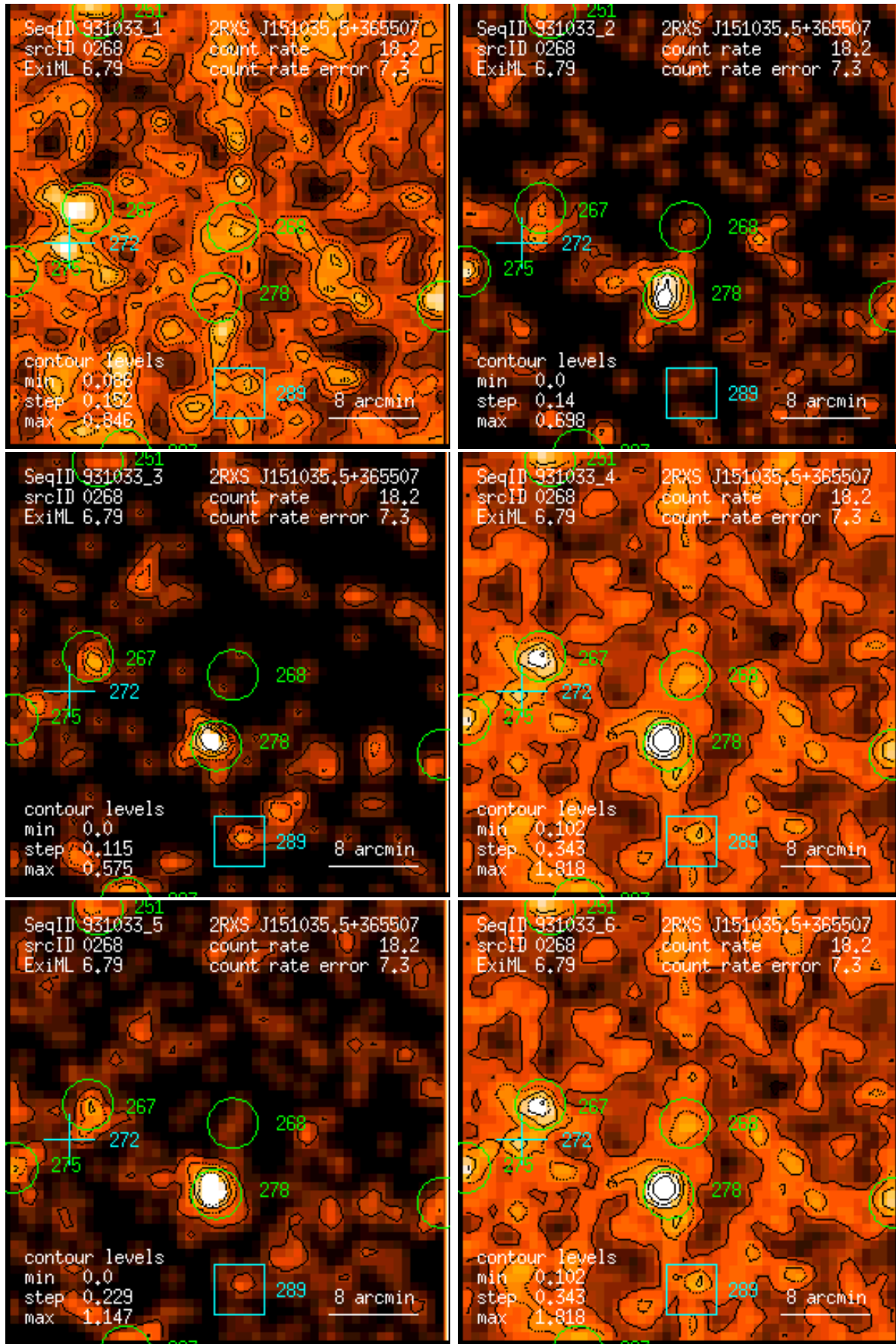
Figure 268: RASS 931033: detection 0268: band rate images, Gaussian filter: (1) PSPC channels 11 – 41, (2) 52 – 90, (3) 91 – 201, (4) 11 – 235, (5) 52 – 201, (6) 11 – 201. Broad band rates in counts/ks. Band rate contour levels in counts/ks/arcmin 2 .
