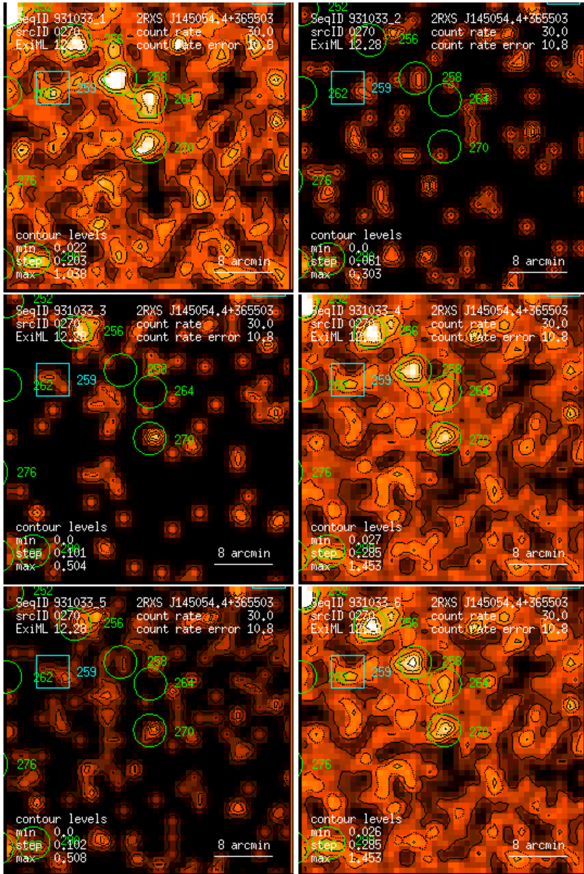
Figure 270: RASS 931033: detection 0270: band rate images, Gaussian filter: (1) PSPC channels 11 – 41, (2) 52 – 90, (3) 91 – 201, (4) 11 – 235, (5) 52 – 201, (6) 11 – 201. Broad band rates in counts/ks. Band rate contour levels in counts/ks/arcmin 2 .
