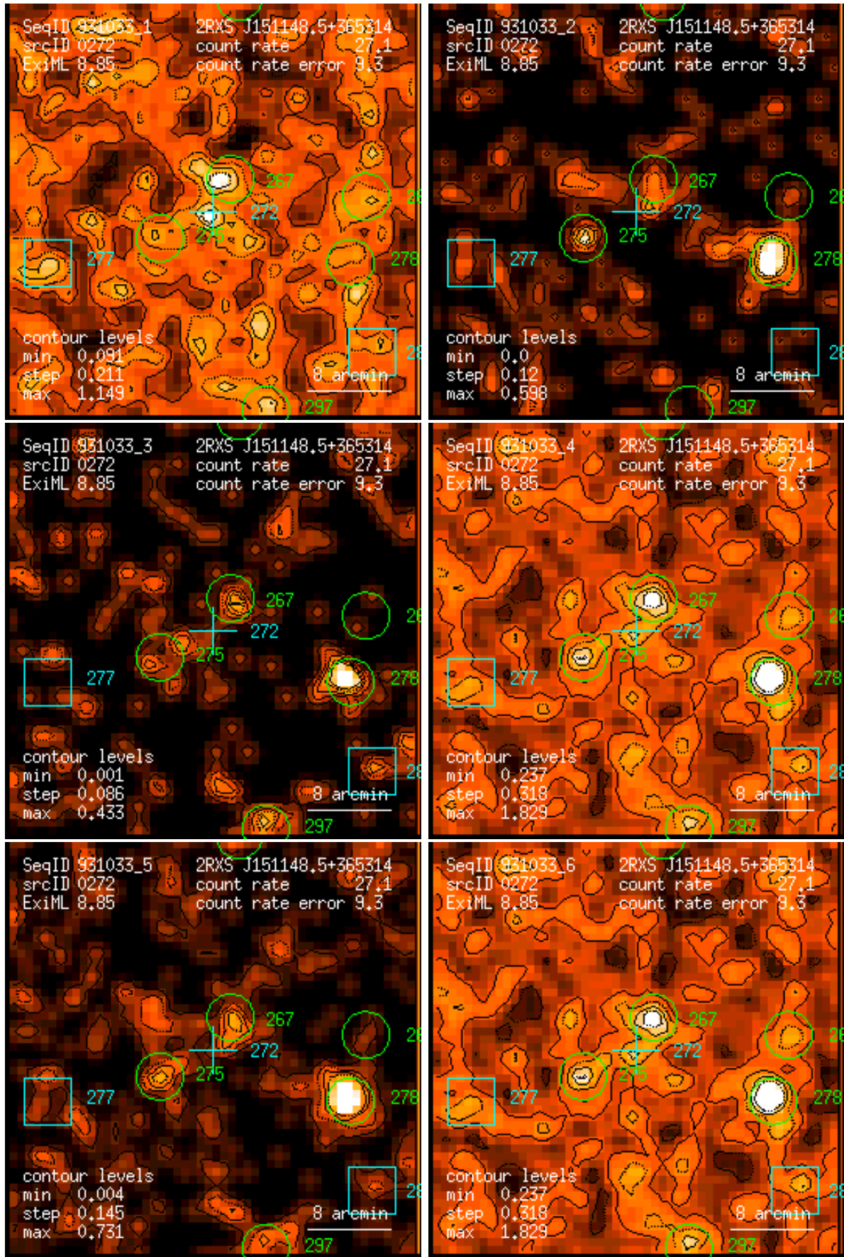
Figure 272: RASS 931033: detection 0272: band rate images, Gaussian filter: (1) PSPC channels 11 – 41, (2) 52 – 90, (3) 91 – 201, (4) 11 – 235, (5) 52 – 201, (6) 11 – 201. Broad band rates in counts/ks. Band rate contour levels in counts/ks/arcmin 2 .
