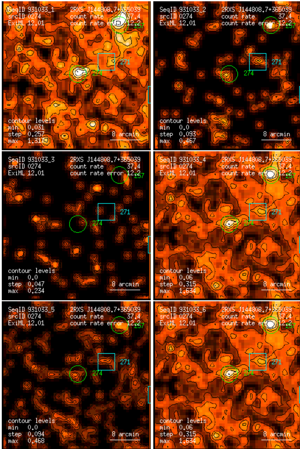
Figure 274: RASS 931033: detection 0274: band rate images, Gaussian filter: (1) PSPC channels 11 – 41, (2) 52 – 90, (3) 91 – 201, (4) 11 – 235, (5) 52 – 201, (6) 11 – 201. Broad band rates in counts/ks. Band rate contour levels in counts/ks/arcmin 2 .
