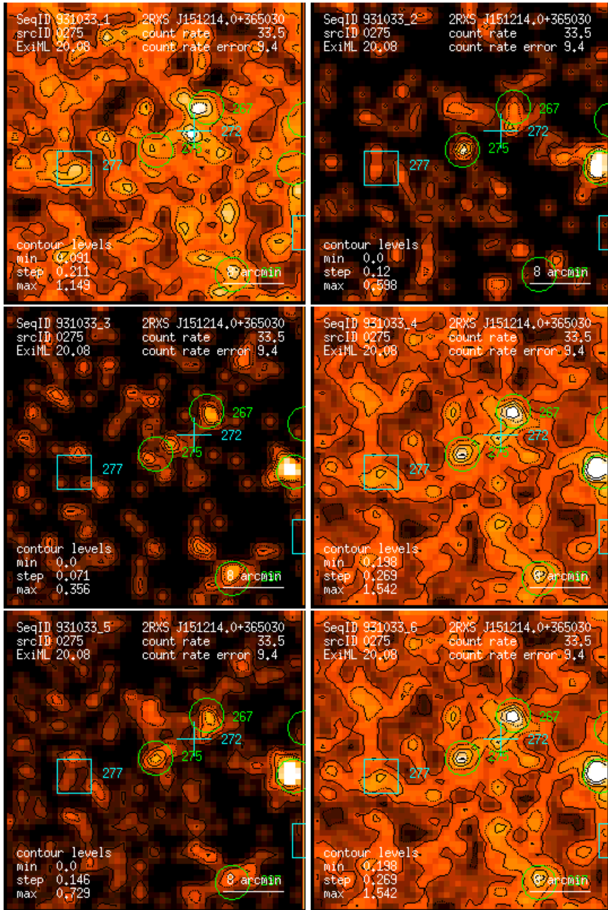
Figure 275: RASS 931033: detection 0275: band rate images, Gaussian filter: (1) PSPC channels 11 – 41, (2) 52 – 90, (3) 91 – 201, (4) 11 – 235, (5) 52 – 201, (6) 11 – 201. Broad band rates in counts/ks. Band rate contour levels in counts/ks/arcmin 2 .
