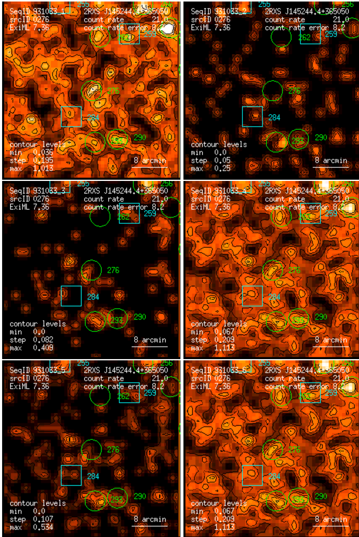
Figure 276: RASS 931033: detection 0276: band rate images, Gaussian filter: (1) PSPC channels 11 – 41, (2) 52 – 90, (3) 91 – 201, (4) 11 – 235, (5) 52 – 201, (6) 11 – 201. Broad band rates in counts/ks. Band rate contour levels in counts/ks/arcmin 2 .
