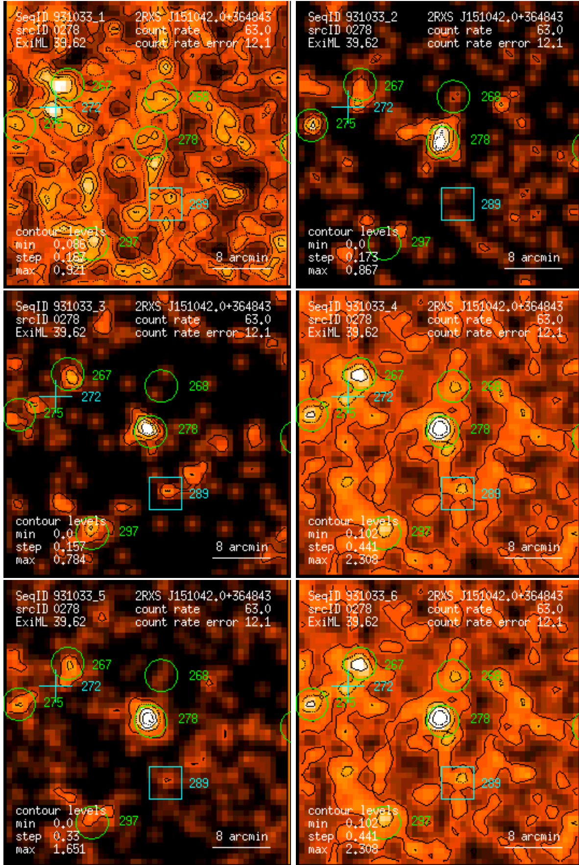
Figure 278: RASS 931033: detection 0278: band rate images, Gaussian filter: (1) PSPC channels 11 – 41, (2) 52 – 90, (3) 91 – 201, (4) 11 – 235, (5) 52 – 201, (6) 11 – 201. Broad band rates in counts/ks. Band rate contour levels in counts/ks/arcmin 2 .
