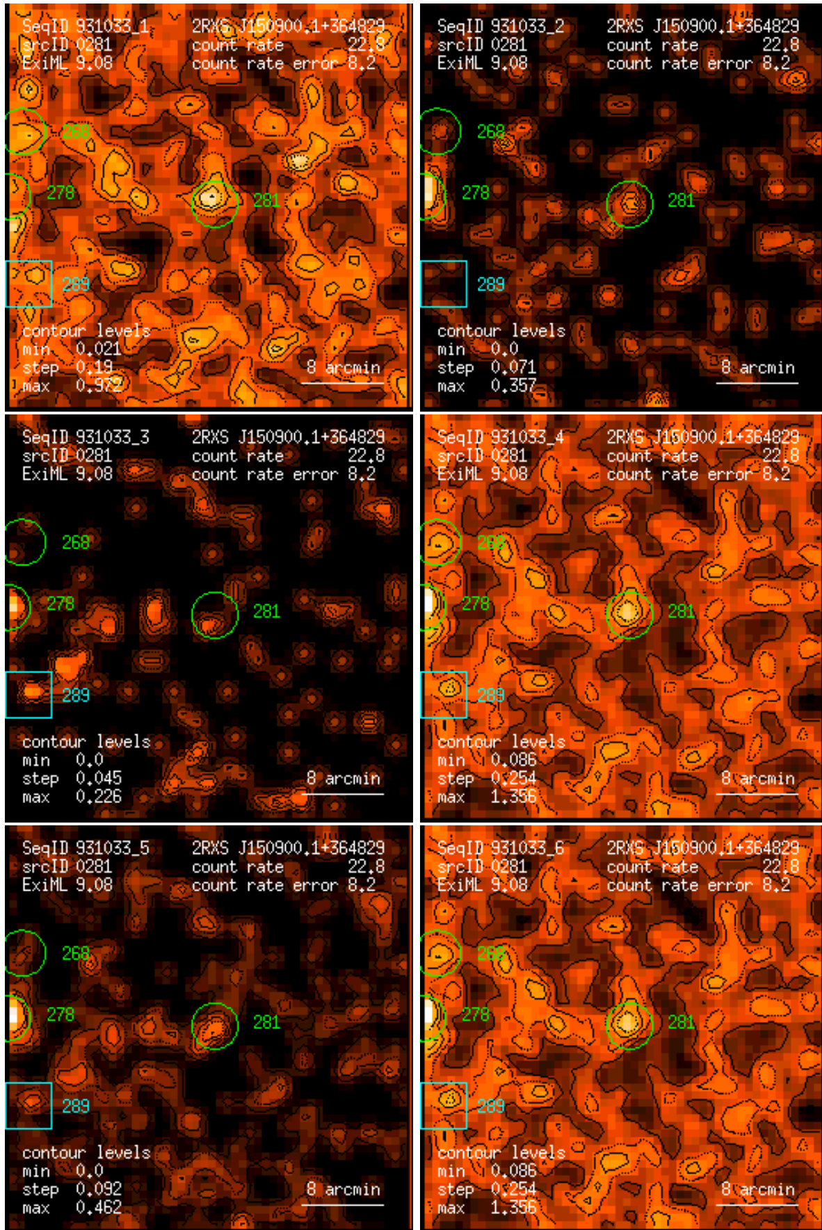
Figure 281: RASS 931033: detection 0281: band rate images, Gaussian filter: (1) PSPC channels 11 – 41, (2) 52 – 90, (3) 91 – 201, (4) 11 – 235, (5) 52 – 201, (6) 11 – 201. Broad band rates in counts/ks. Band rate contour levels in counts/ks/arcmin 2 .
