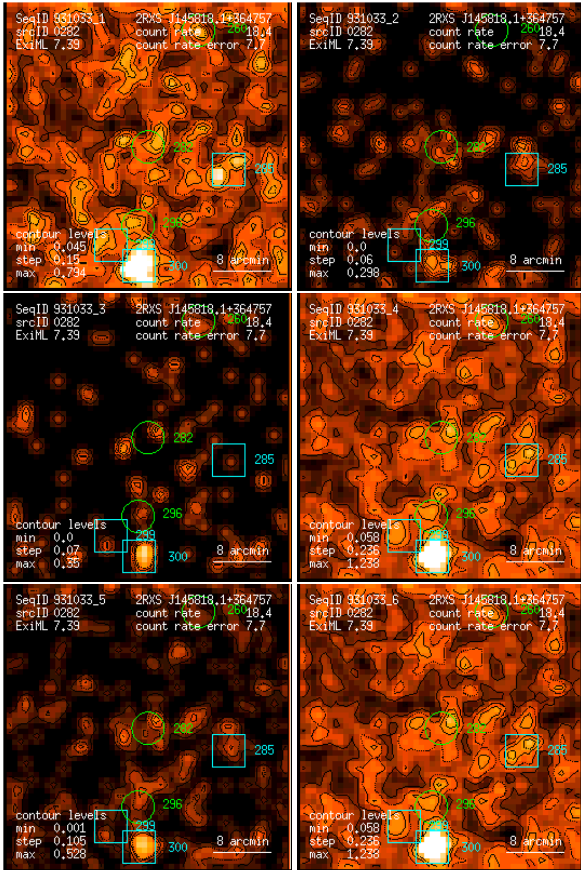
Figure 282: RASS 931033: detection 0282: band rate images, Gaussian filter: (1) PSPC channels 11 – 41, (2) 52 – 90, (3) 91 – 201, (4) 11 – 235, (5) 52 – 201, (6) 11 – 201. Broad band rates in counts/ks. Band rate contour levels in counts/ks/arcmin 2 .
