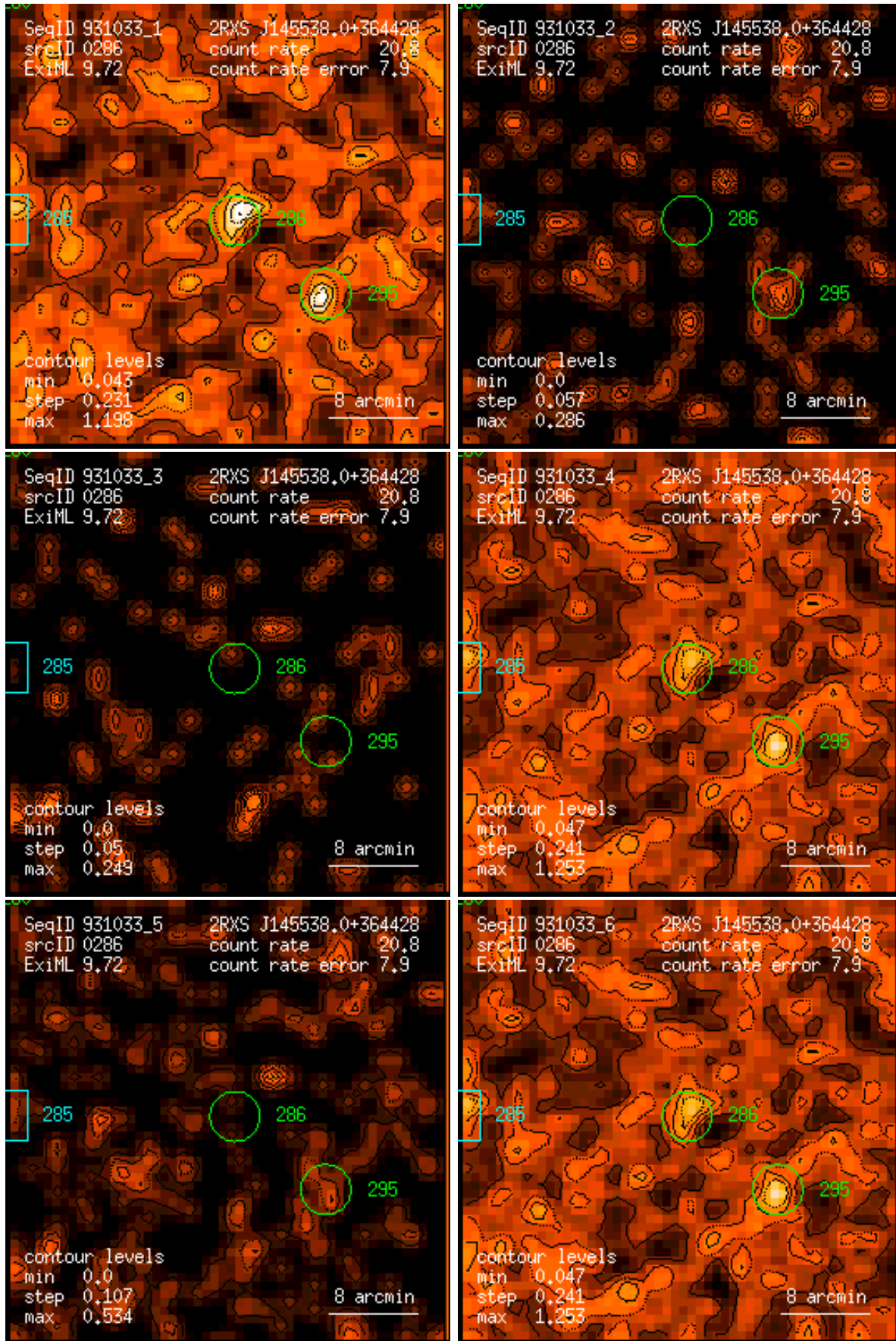
Figure 286: RASS 931033: detection 0286: band rate images, Gaussian filter: (1) PSPC channels 11 – 41, (2) 52 – 90, (3) 91 – 201, (4) 11 – 235, (5) 52 – 201, (6) 11 – 201. Broad band rates in counts/ks. Band rate contour levels in counts/ks/arcmin 2 .
