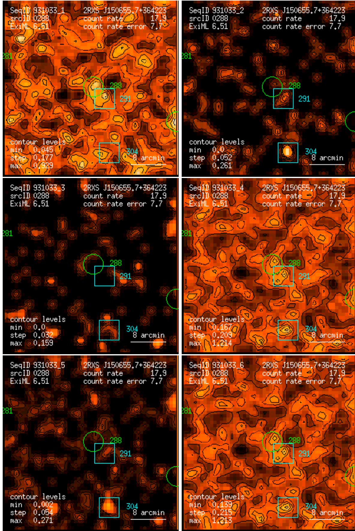
Figure 288: RASS 931033: detection 0288: band rate images, Gaussian filter: (1) PSPC channels 11 – 41, (2) 52 – 90, (3) 91 – 201, (4) 11 – 235, (5) 52 – 201, (6) 11 – 201. Broad band rates in counts/ks. Band rate contour levels in counts/ks/arcmin 2 .
