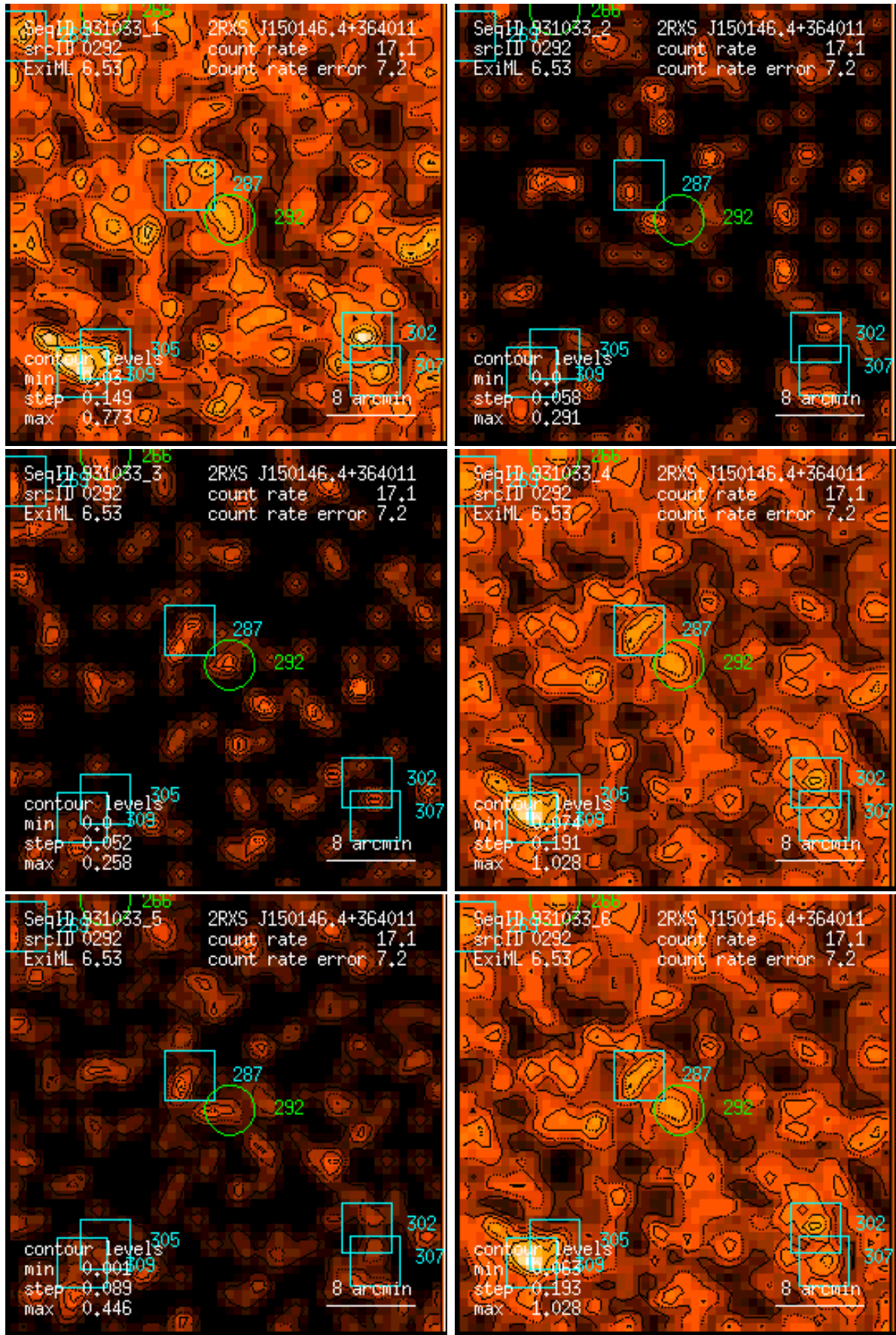
Figure 292: RASS 931033: detection 0292: band rate images, Gaussian filter: (1) PSPC channels 11 – 41, (2) 52 – 90, (3) 91 – 201, (4) 11 – 235, (5) 52 – 201, (6) 11 – 201. Broad band rates in counts/ks. Band rate contour levels in counts/ks/arcmin 2 .
