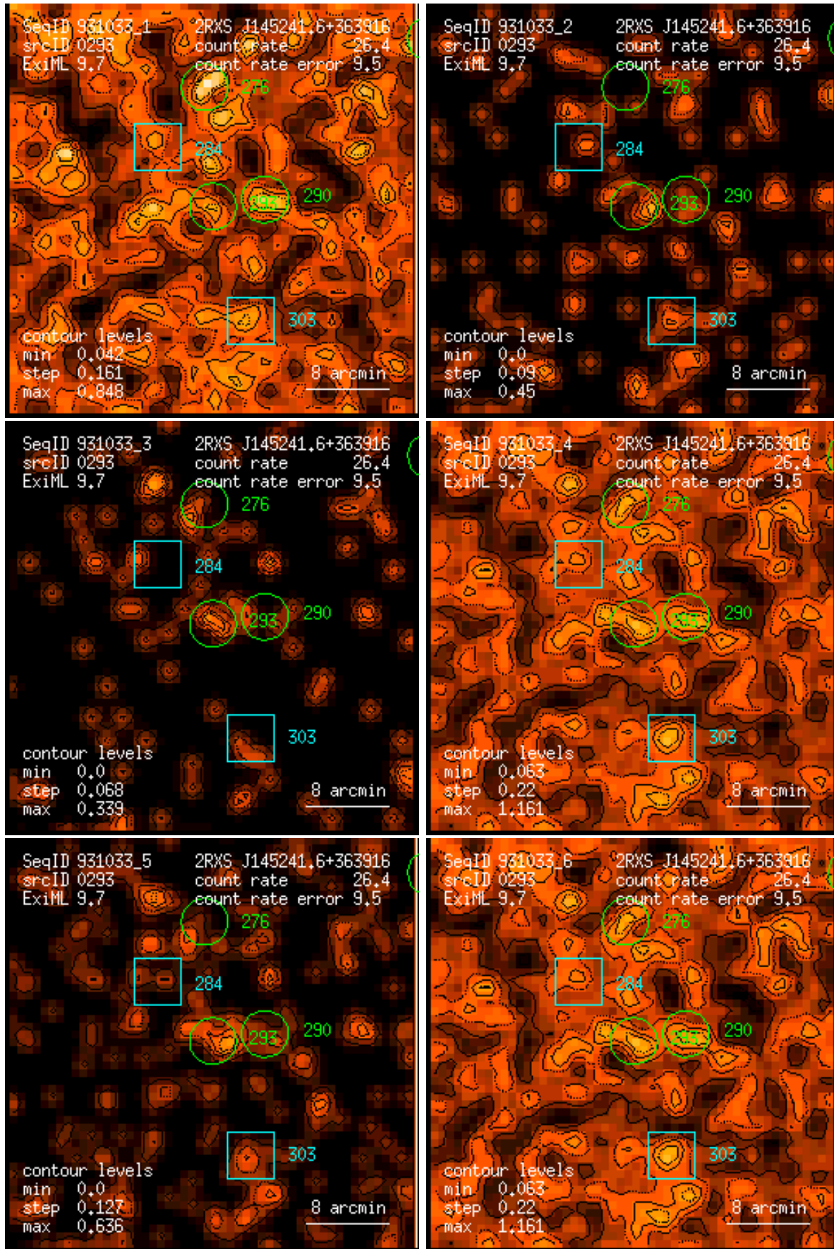
Figure 293: RASS 931033: detection 0293: band rate images, Gaussian filter: (1) PSPC channels 11 – 41, (2) 52 – 90, (3) 91 – 201, (4) 11 – 235, (5) 52 – 201, (6) 11 – 201. Broad band rates in counts/ks. Band rate contour levels in counts/ks/arcmin 2 .
