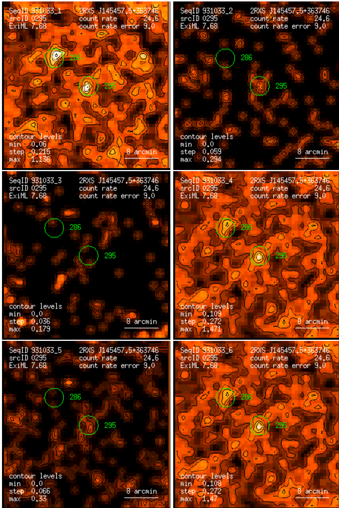
Figure 295: RASS 931033: detection 0295: band rate images, Gaussian filter: (1) PSPC channels 11 – 41, (2) 52 – 90, (3) 91 – 201, (4) 11 – 235, (5) 52 – 201, (6) 11 – 201. Broad band rates in counts/ks. Band rate contour levels in counts/ks/arcmin 2 .
