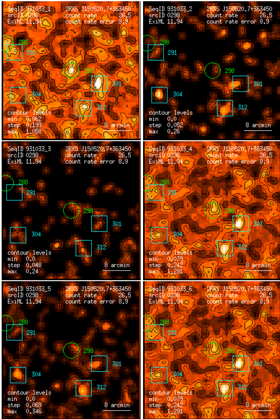
Figure 298: RASS 931033: detection 0298: band rate images, Gaussian filter: (1) PSPC channels 11 – 41, (2) 52 – 90, (3) 91 – 201, (4) 11 – 235, (5) 52 – 201, (6) 11 – 201. Broad band rates in counts/ks. Band rate contour levels in counts/ks/arcmin 2 .
