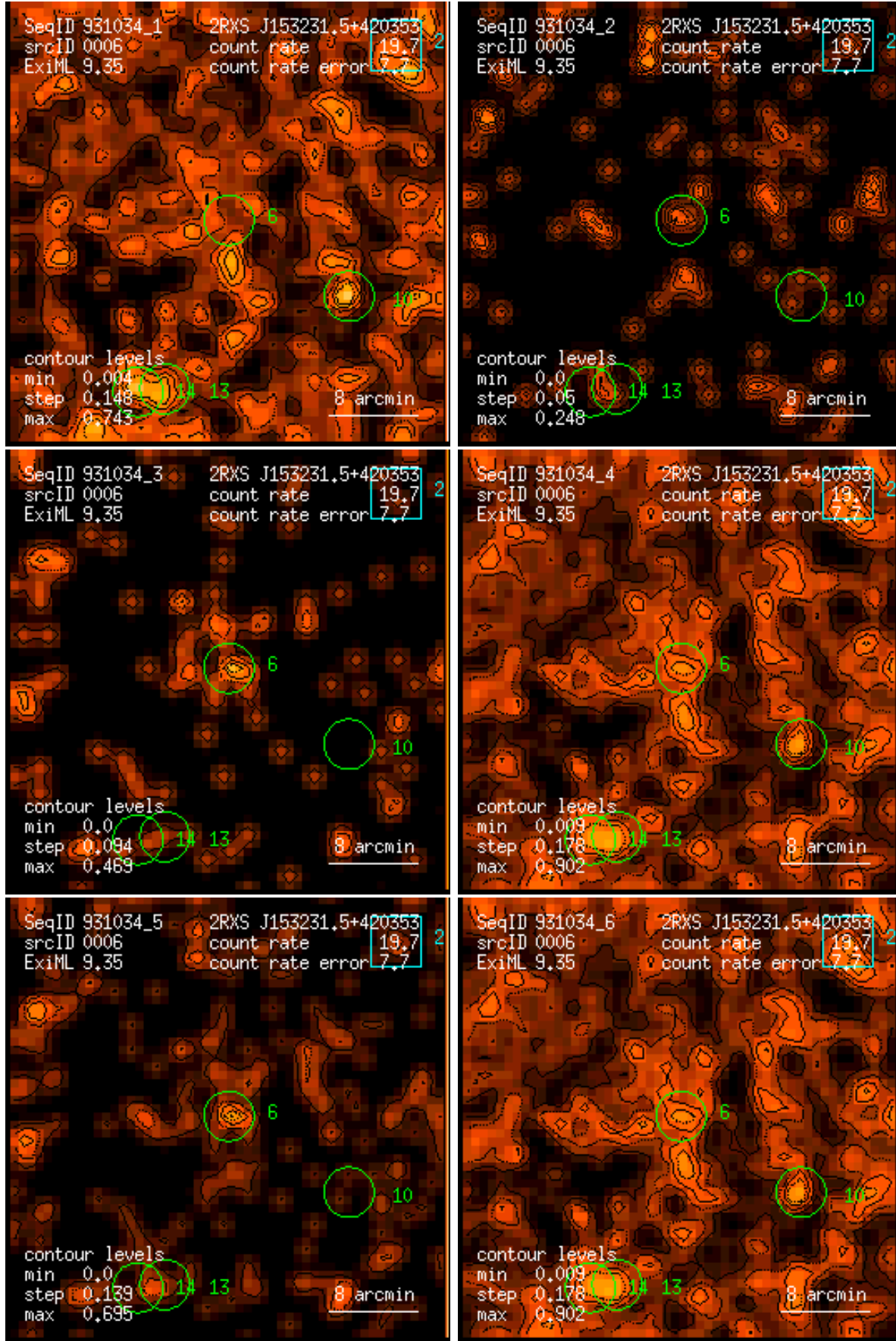
Figure 6: RASS 931034: detection 0006: band rate images, Gaussian filter: (1) PSPC channels 11 – 41, (2) 52 – 90, (3) 91 – 201, (4) 11 – 235, (5) 52 – 201, (6) 11 – 201. Broad band rates in counts/ks. Band rate contour levels in counts/ks/arcmin 2 .
