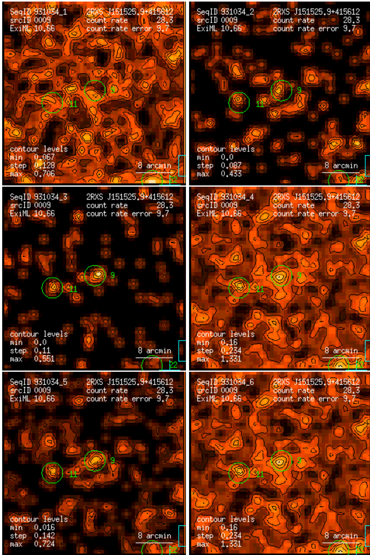
Figure 9: RASS 931034: detection 0009: band rate images, Gaussian filter: (1) PSPC channels 11 – 41, (2) 52 – 90, (3) 91 – 201, (4) 11 – 235, (5) 52 – 201, (6) 11 – 201. Broad band rates in counts/ks. Band rate contour levels in counts/ks/arcmin 2 .
