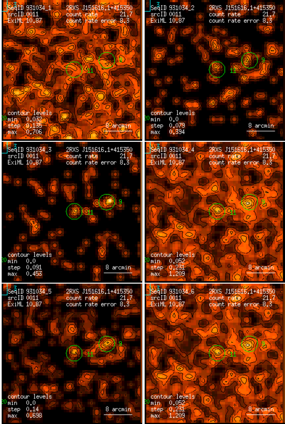
Figure 11: RASS 931034: detection 0011: band rate images, Gaussian filter: (1) PSPC channels 11 – 41, (2) 52 – 90, (3) 91 – 201, (4) 11 – 235, (5) 52 – 201, (6) 11 – 201. Broad band rates in counts/ks. Band rate contour levels in counts/ks/arcmin 2 .
