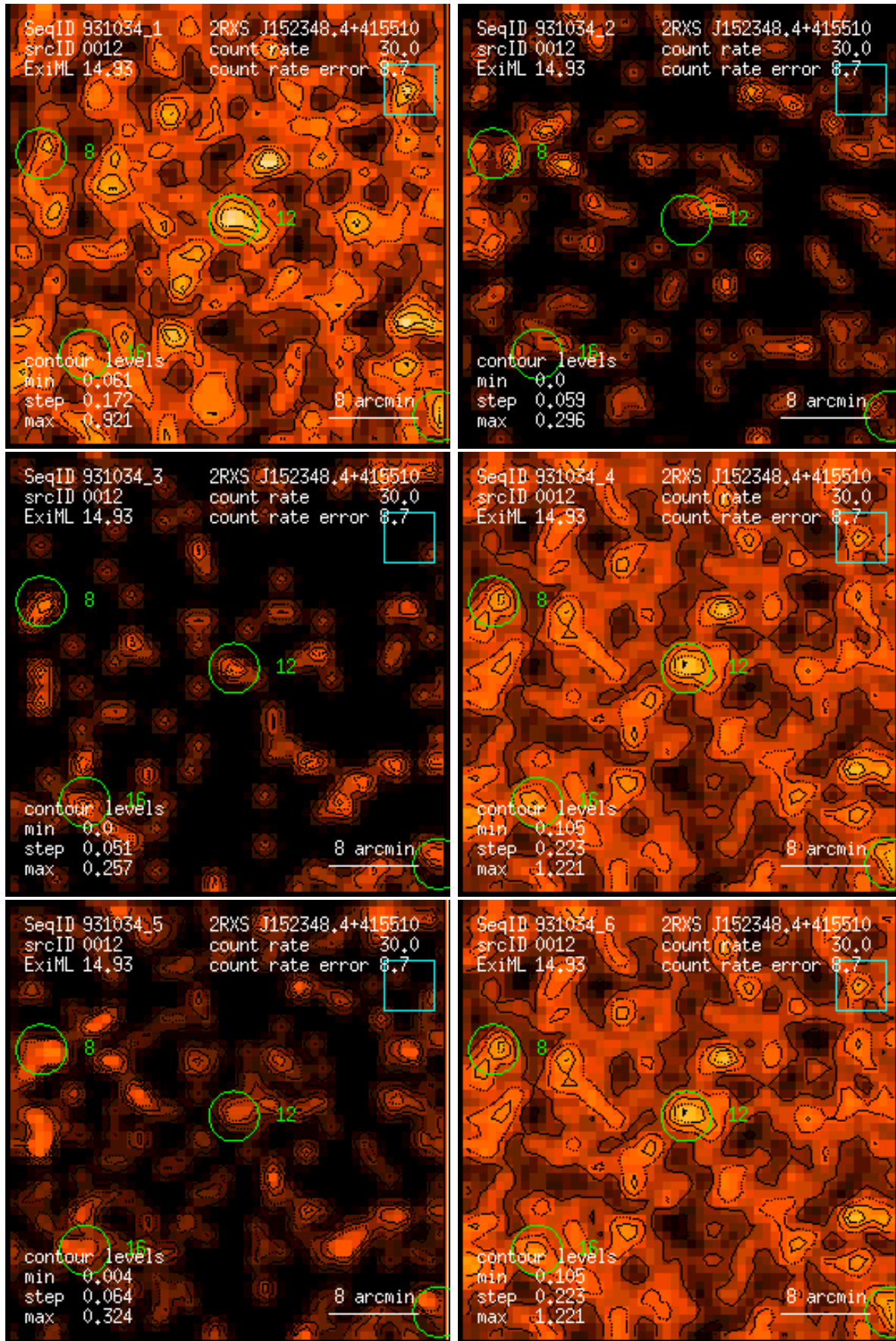
Figure 12: RASS 931034: detection 0012: band rate images, Gaussian filter: (1) PSPC channels 11 – 41, (2) 52 – 90, (3) 91 – 201, (4) 11 – 235, (5) 52 – 201, (6) 11 – 201. Broad band rates in counts/ks. Band rate contour levels in counts/ks/arcmin 2 .
