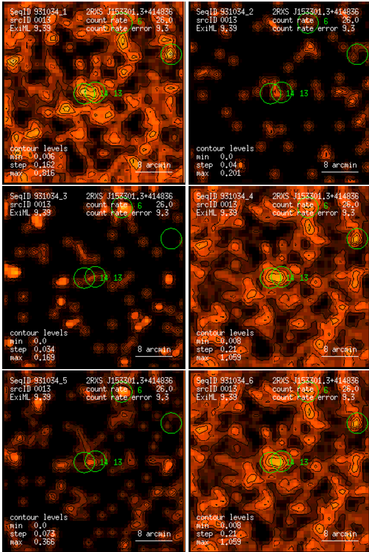
Figure 13: RASS 931034: detection 0013: band rate images, Gaussian filter: (1) PSPC channels 11 – 41, (2) 52 – 90, (3) 91 – 201, (4) 11 – 235, (5) 52 – 201, (6) 11 – 201. Broad band rates in counts/ks. Band rate contour levels in counts/ks/arcmin 2 .
