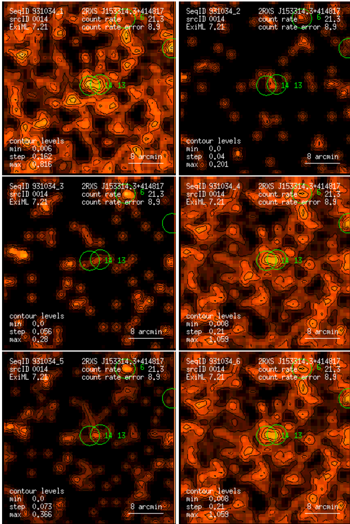
Figure 14: RASS 931034: detection 0014: band rate images, Gaussian filter: (1) PSPC channels 11 – 41, (2) 52 – 90, (3) 91 – 201, (4) 11 – 235, (5) 52 – 201, (6) 11 – 201. Broad band rates in counts/ks. Band rate contour levels in counts/ks/arcmin 2 .
