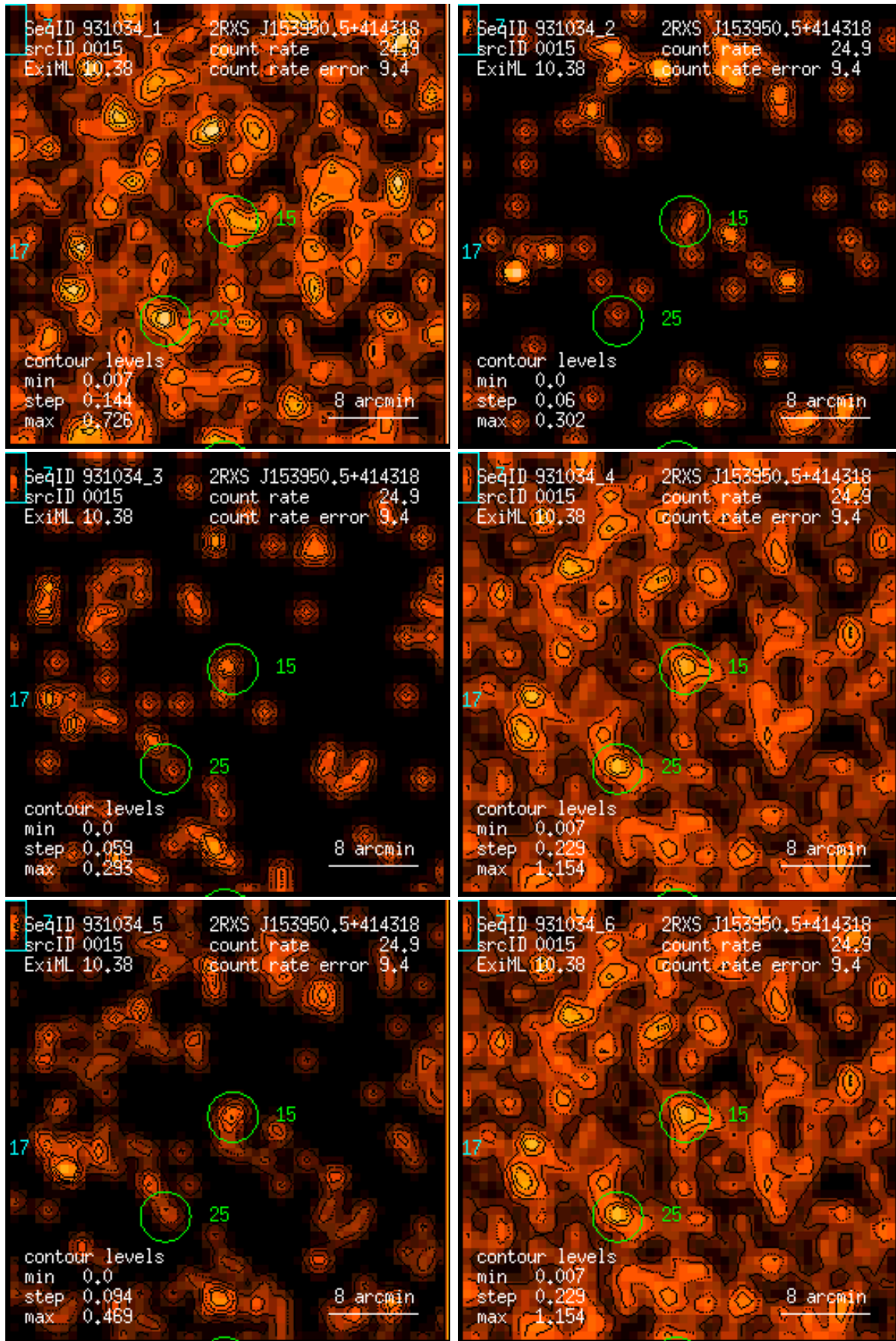
Figure 15: RASS 931034: detection 0015: band rate images, Gaussian filter: (1) PSPC channels 11 – 41, (2) 52 – 90, (3) 91 – 201, (4) 11 – 235, (5) 52 – 201, (6) 11 – 201. Broad band rates in counts/ks. Band rate contour levels in counts/ks/arcmin 2 .
