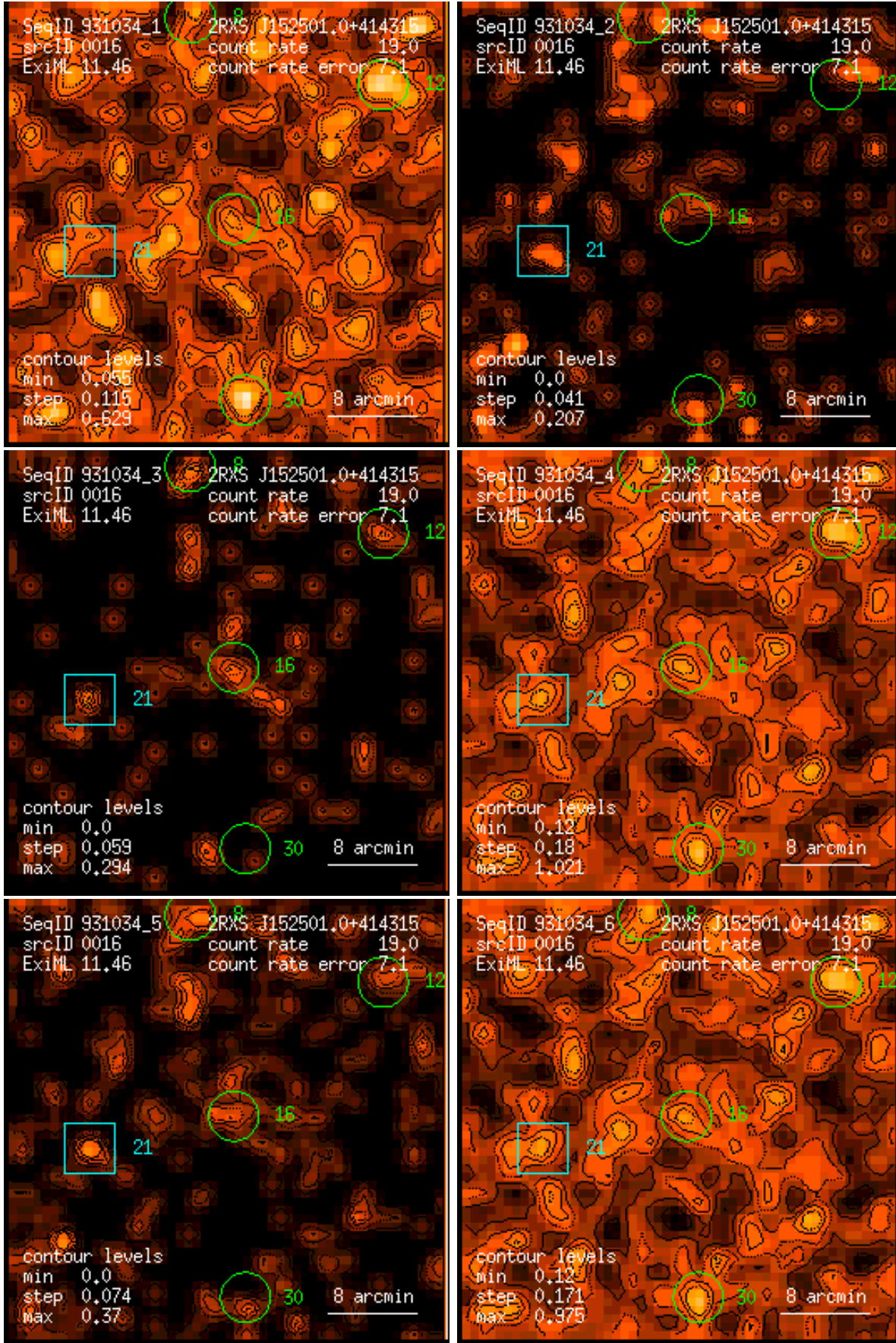
Figure 16: RASS 931034: detection 0016: band rate images, Gaussian filter: (1) PSPC channels 11 – 41, (2) 52 – 90, (3) 91 – 201, (4) 11 – 235, (5) 52 – 201, (6) 11 – 201. Broad band rates in counts/ks. Band rate contour levels in counts/ks/arcmin 2 .
