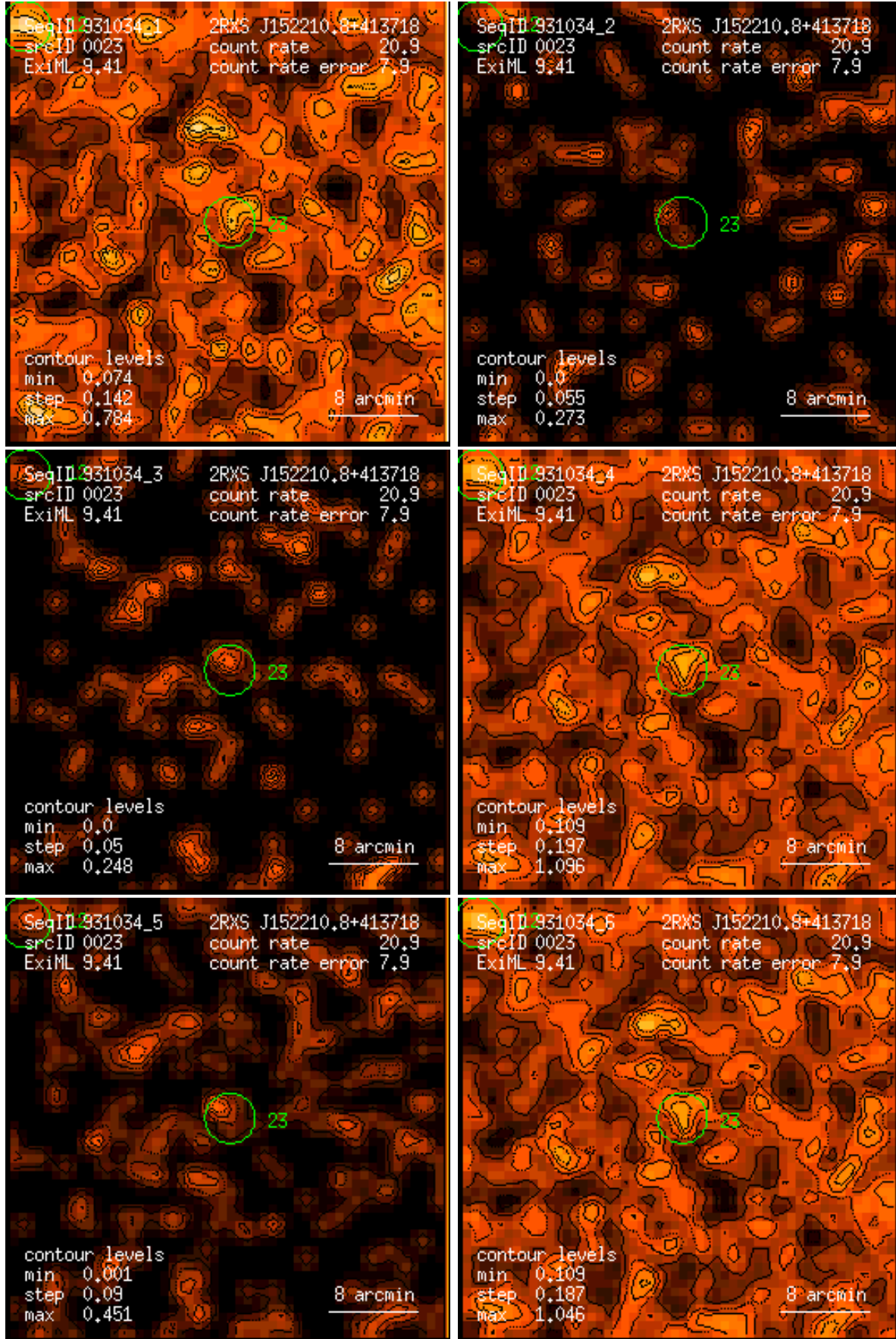
Figure 23: RASS 931034: detection 0023: band rate images, Gaussian filter: (1) PSPC channels 11 – 41, (2) 52 – 90, (3) 91 – 201, (4) 11 – 235, (5) 52 – 201, (6) 11 – 201. Broad band rates in counts/ks. Band rate contour levels in counts/ks/arcmin 2 .
