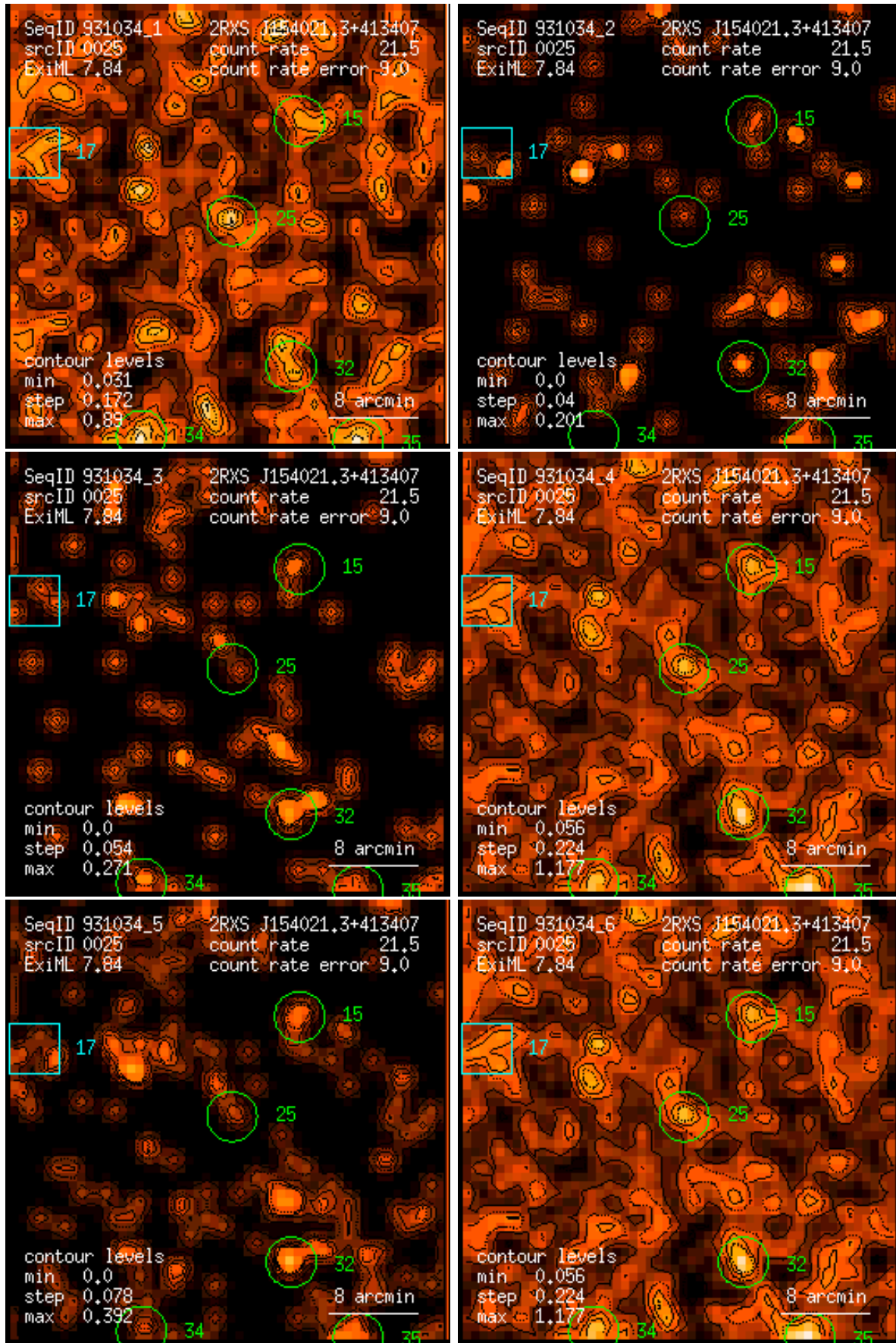
Figure 25: RASS 931034: detection 0025: band rate images, Gaussian filter: (1) PSPC channels 11 – 41, (2) 52 – 90, (3) 91 – 201, (4) 11 – 235, (5) 52 – 201, (6) 11 – 201. Broad band rates in counts/ks. Band rate contour levels in counts/ks/arcmin 2 .
