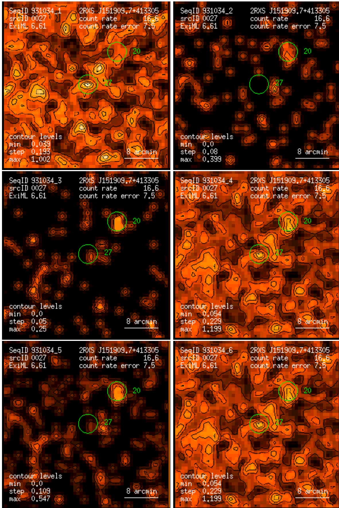
Figure 27: RASS 931034: detection 0027: band rate images, Gaussian filter: (1) PSPC channels 11 – 41, (2) 52 – 90, (3) 91 – 201, (4) 11 – 235, (5) 52 – 201, (6) 11 – 201. Broad band rates in counts/ks. Band rate contour levels in counts/ks/arcmin 2 .
