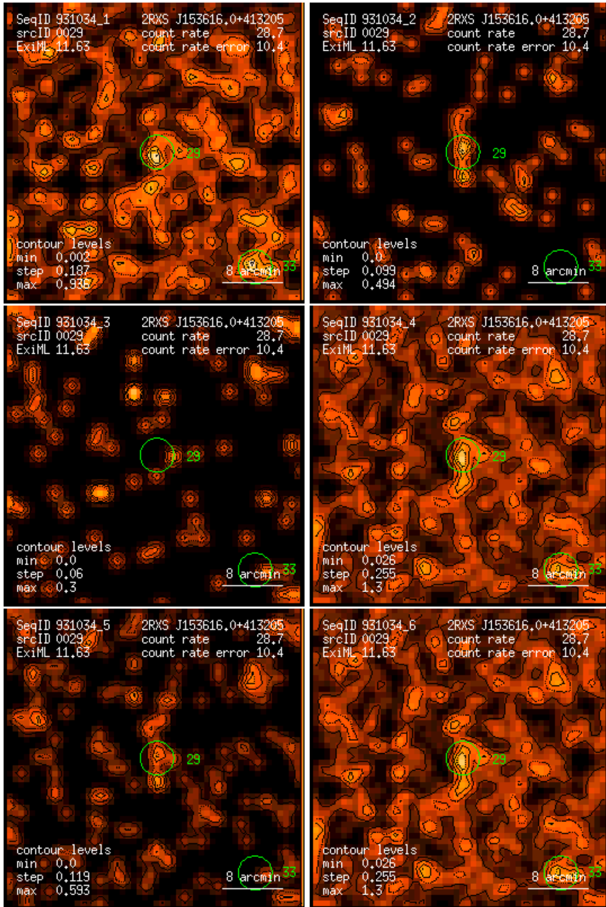
Figure 29: RASS 931034: detection 0029: band rate images, Gaussian filter: (1) PSPC channels 11 – 41, (2) 52 – 90, (3) 91 – 201, (4) 11 – 235, (5) 52 – 201, (6) 11 – 201. Broad band rates in counts/ks. Band rate contour levels in counts/ks/arcmin 2 .
