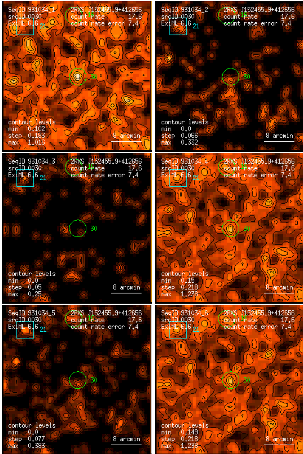
Figure 30: RASS 931034: detection 0030: band rate images, Gaussian filter: (1) PSPC channels 11 – 41, (2) 52 – 90, (3) 91 – 201, (4) 11 – 235, (5) 52 – 201, (6) 11 – 201. Broad band rates in counts/ks. Band rate contour levels in counts/ks/arcmin 2 .
