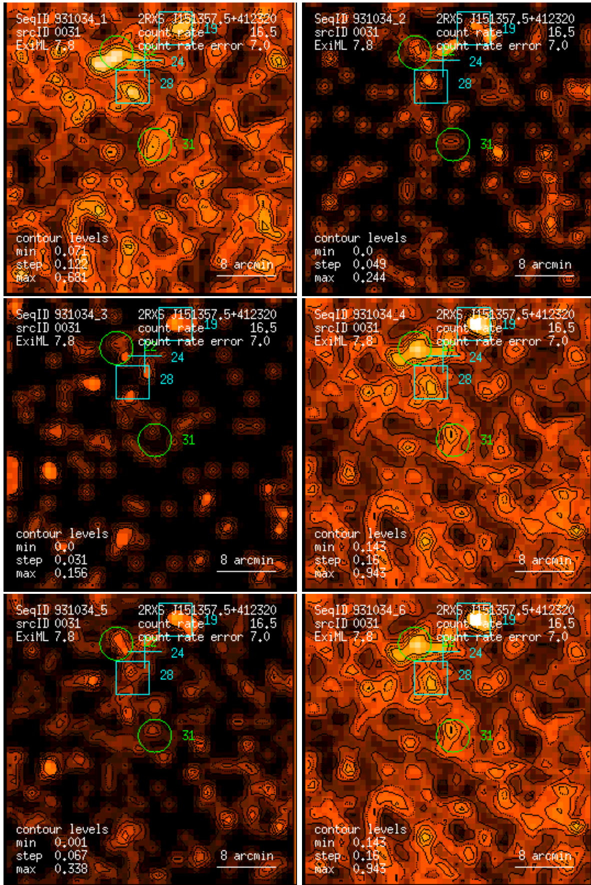
Figure 31: RASS 931034: detection 0031: band rate images, Gaussian filter: (1) PSPC channels 11 – 41, (2) 52 – 90, (3) 91 – 201, (4) 11 – 235, (5) 52 – 201, (6) 11 – 201. Broad band rates in counts/ks. Band rate contour levels in counts/ks/arcmin 2 .
