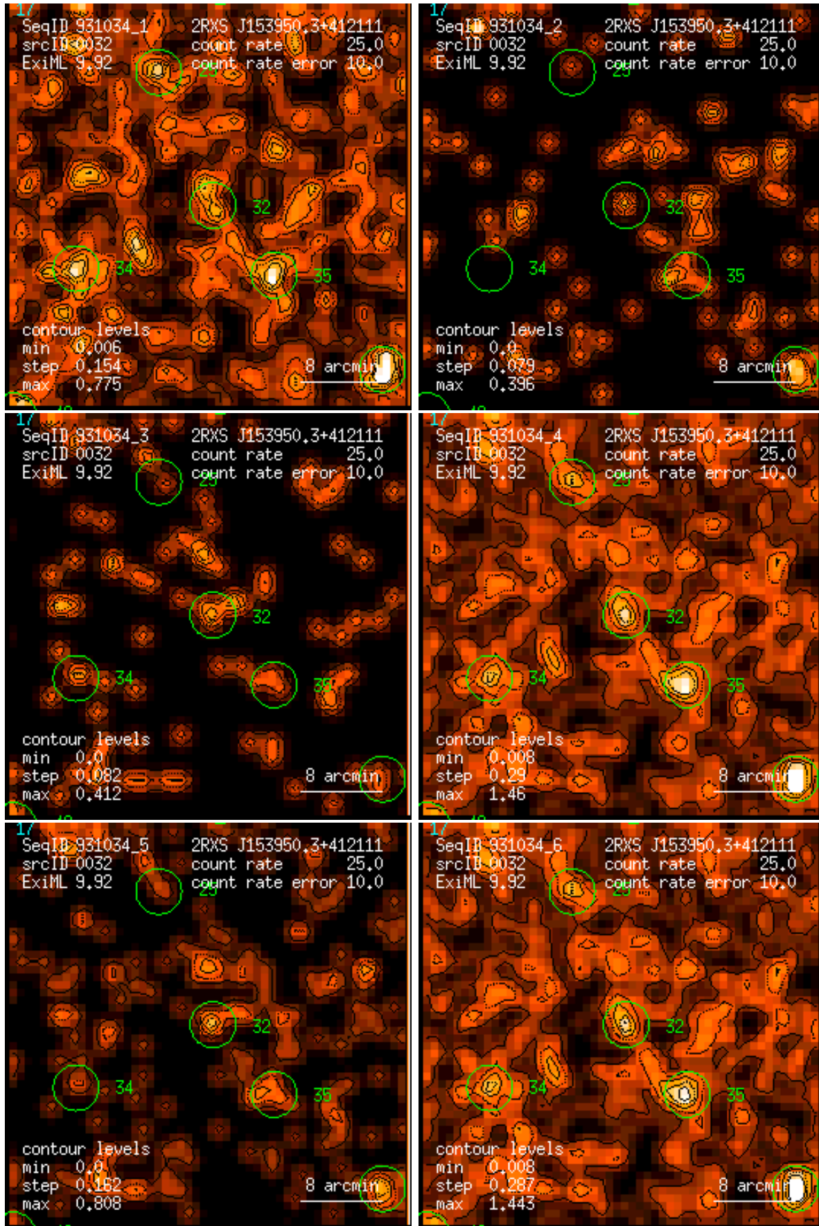
Figure 32: RASS 931034: detection 0032: band rate images, Gaussian filter: (1) PSPC channels 11 – 41, (2) 52 – 90, (3) 91 – 201, (4) 11 – 235, (5) 52 – 201, (6) 11 – 201. Broad band rates in counts/ks. Band rate contour levels in counts/ks/arcmin 2 .
