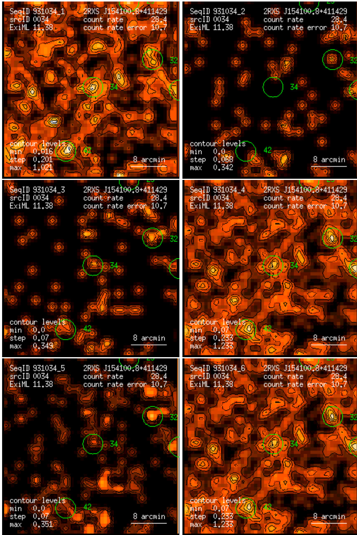
Figure 34: RASS 931034: detection 0034: band rate images, Gaussian filter: (1) PSPC channels 11 – 41, (2) 52 – 90, (3) 91 – 201, (4) 11 – 235, (5) 52 – 201, (6) 11 – 201. Broad band rates in counts/ks. Band rate contour levels in counts/ks/arcmin 2 .
