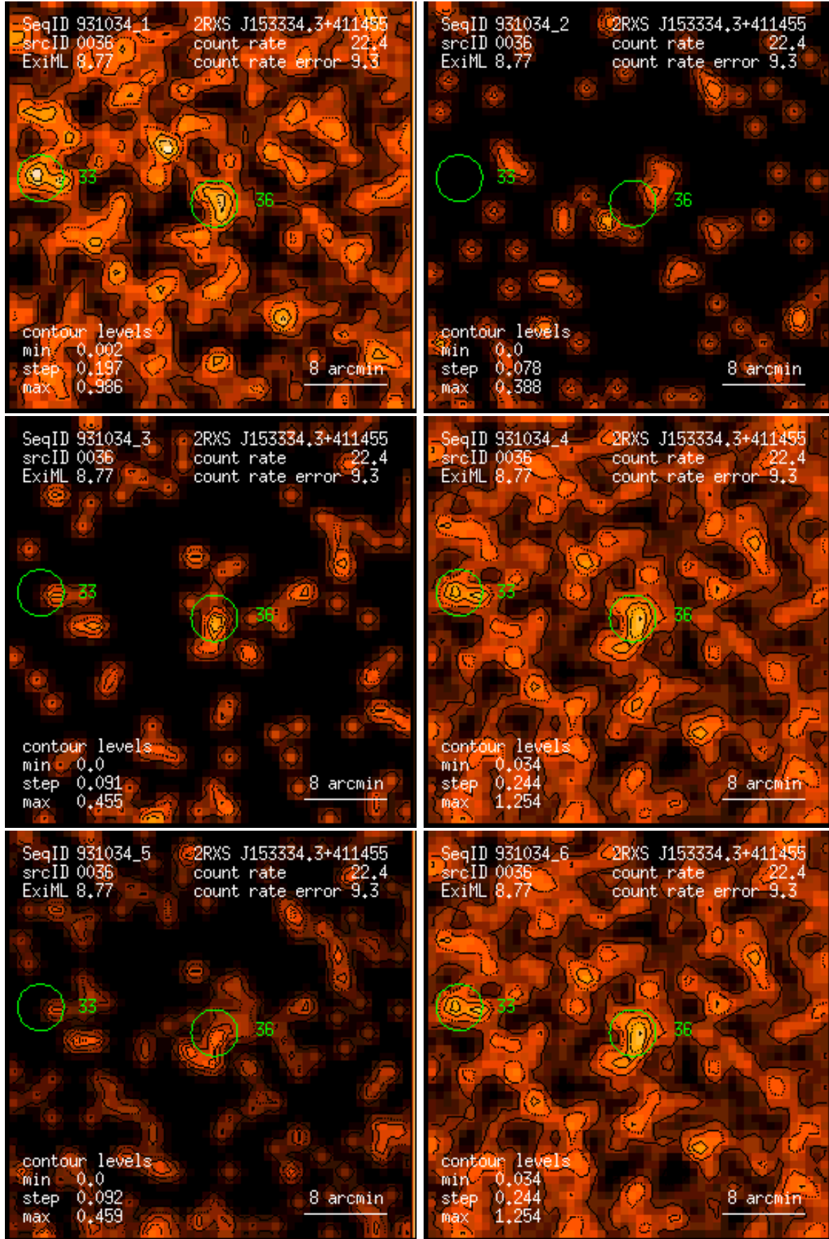
Figure 36: RASS 931034: detection 0036: band rate images, Gaussian filter: (1) PSPC channels 11 – 41, (2) 52 – 90, (3) 91 – 201, (4) 11 – 235, (5) 52 – 201, (6) 11 – 201. Broad band rates in counts/ks. Band rate contour levels in counts/ks/arcmin 2 .
