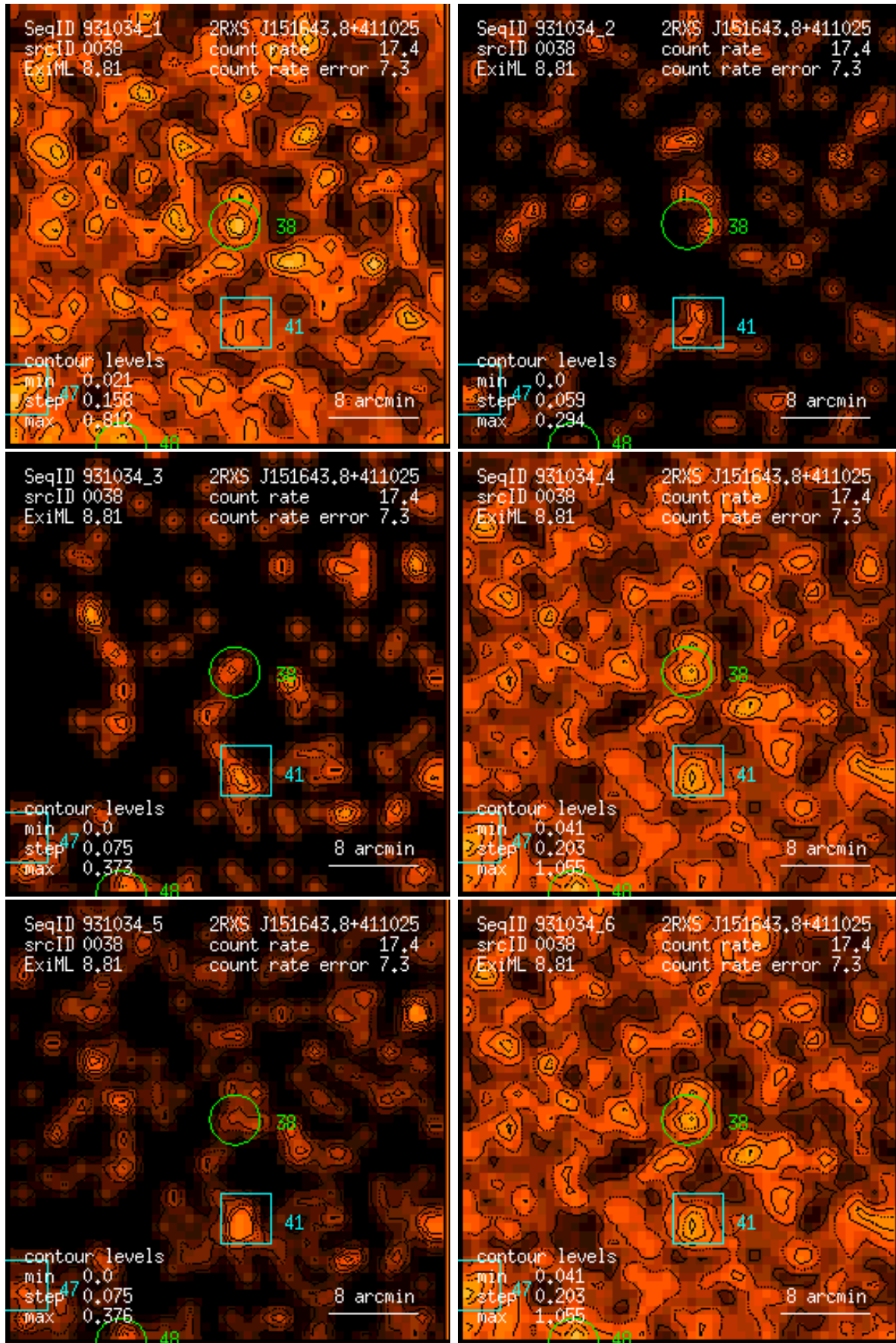
Figure 38: RASS 931034: detection 0038: band rate images, Gaussian filter: (1) PSPC channels 11 – 41, (2) 52 – 90, (3) 91 – 201, (4) 11 – 235, (5) 52 – 201, (6) 11 – 201. Broad band rates in counts/ks. Band rate contour levels in counts/ks/arcmin 2 .
