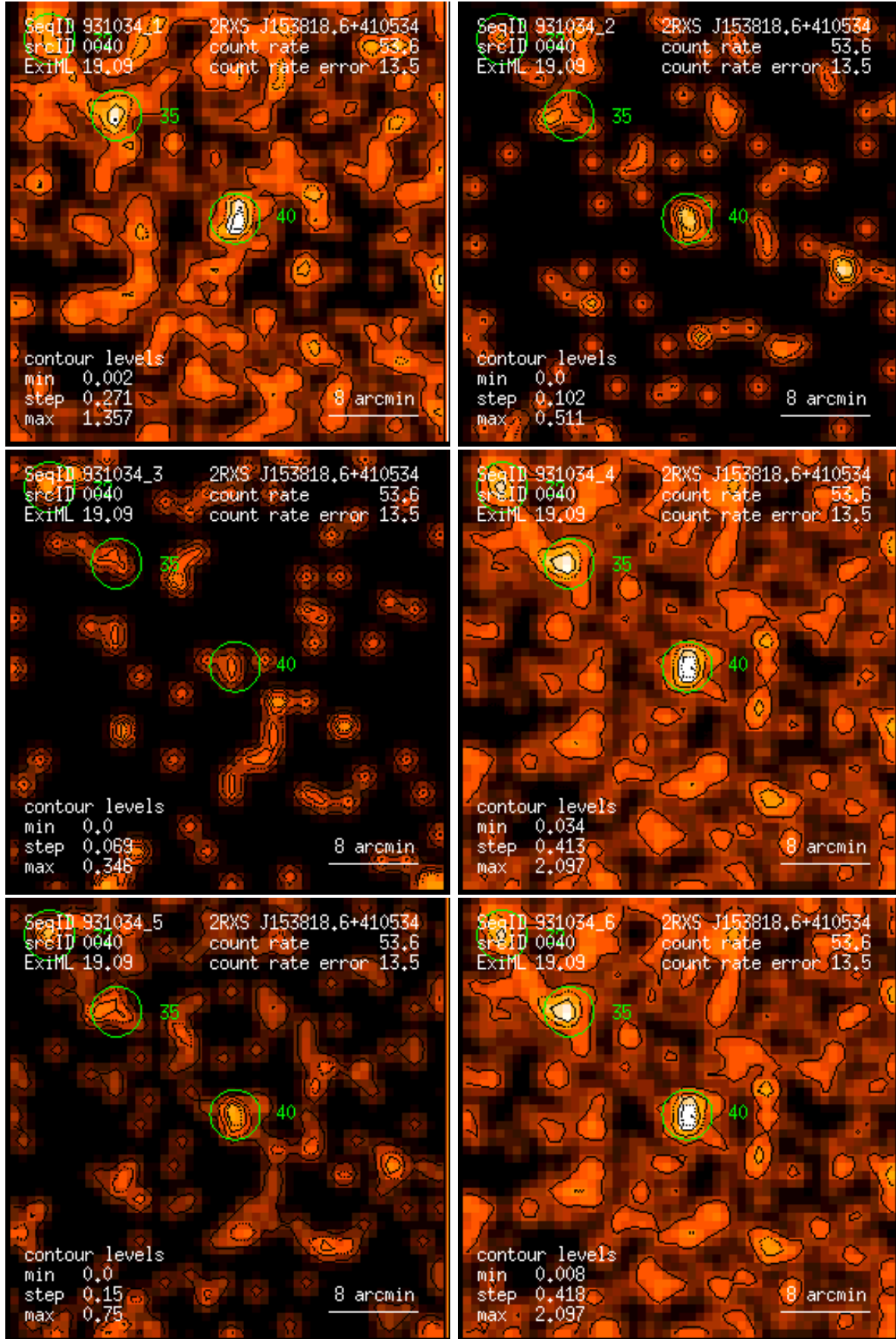
Figure 40: RASS 931034: detection 0040: band rate images, Gaussian filter: (1) PSPC channels 11 – 41, (2) 52 – 90, (3) 91 – 201, (4) 11 – 235, (5) 52 – 201, (6) 11 – 201. Broad band rates in counts/ks. Band rate contour levels in counts/ks/arcmin 2 .
