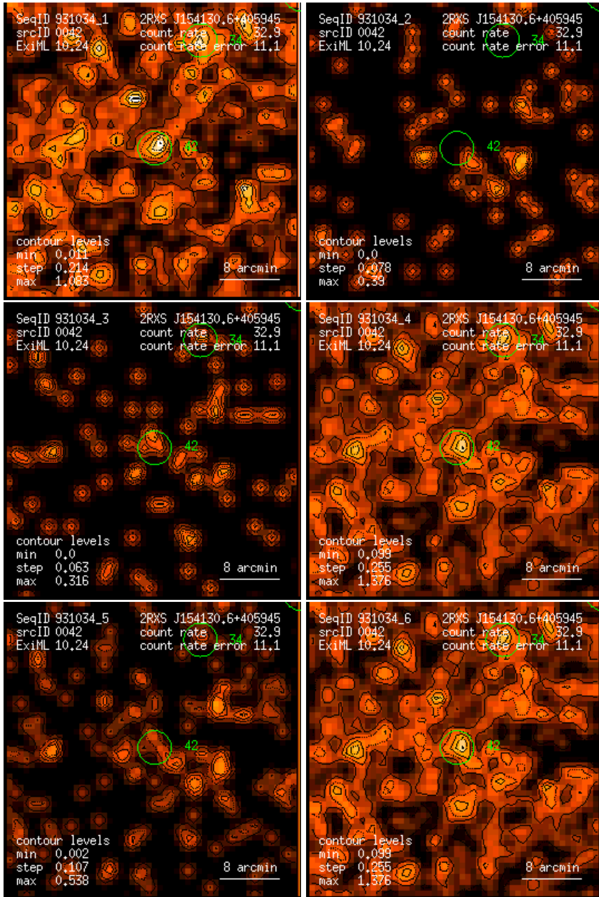
Figure 42: RASS 931034: detection 0042: band rate images, Gaussian filter: (1) PSPC channels 11 – 41, (2) 52 – 90, (3) 91 – 201, (4) 11 – 235, (5) 52 – 201, (6) 11 – 201. Broad band rates in counts/ks. Band rate contour levels in counts/ks/arcmin 2 .
