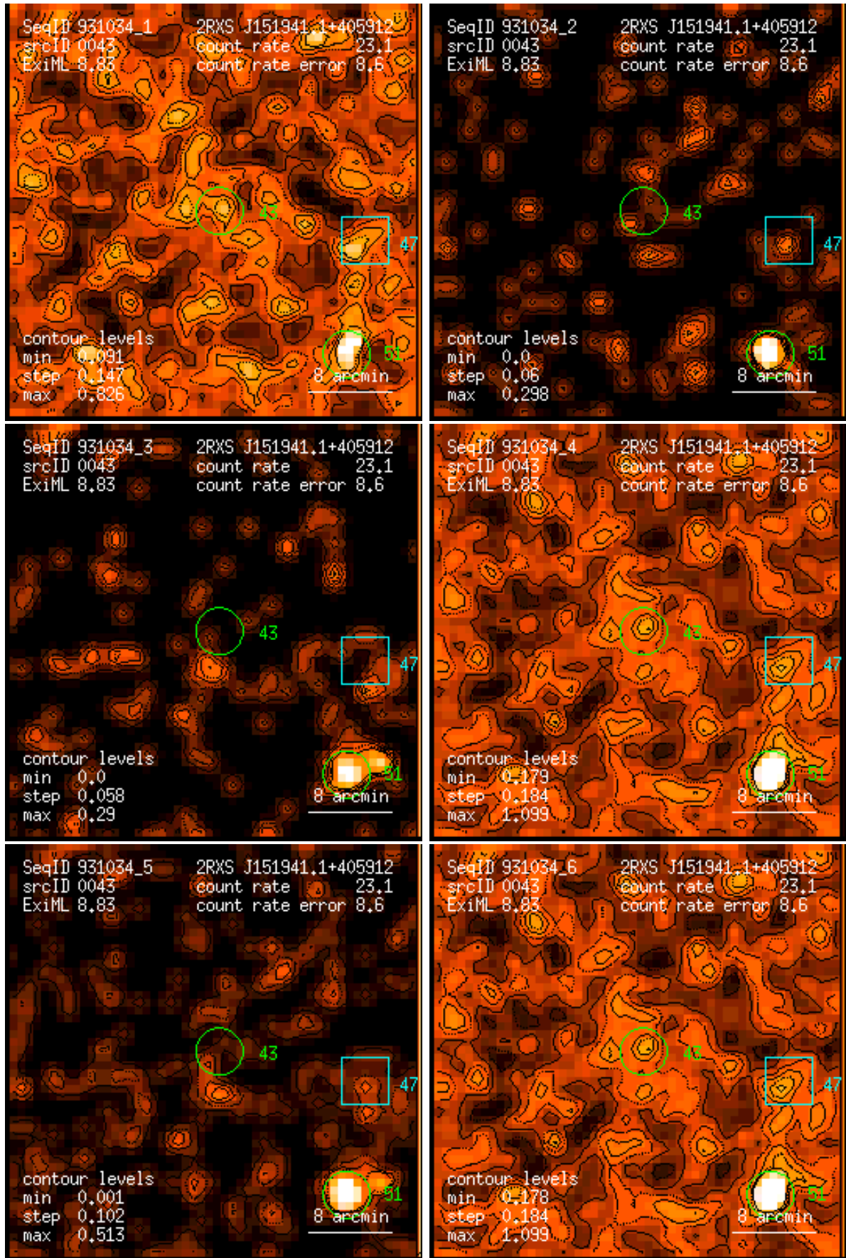
Figure 43: RASS 931034: detection 0043: band rate images, Gaussian filter: (1) PSPC channels 11 – 41, (2) 52 – 90, (3) 91 – 201, (4) 11 – 235, (5) 52 – 201, (6) 11 – 201. Broad band rates in counts/ks. Band rate contour levels in counts/ks/arcmin 2 .
