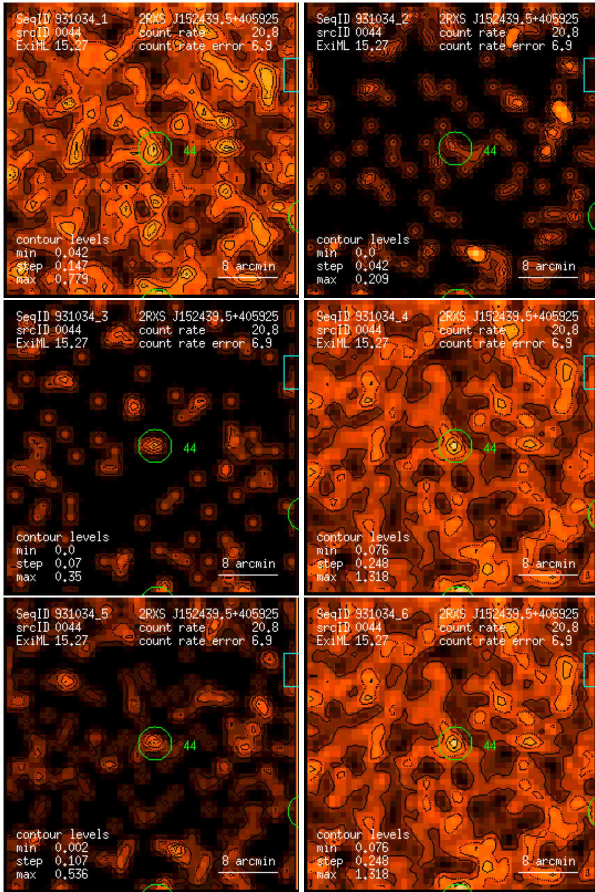
Figure 44: RASS 931034: detection 0044: band rate images, Gaussian filter: (1) PSPC channels 11 – 41, (2) 52 – 90, (3) 91 – 201, (4) 11 – 235, (5) 52 – 201, (6) 11 – 201. Broad band rates in counts/ks. Band rate contour levels in counts/ks/arcmin 2 .
