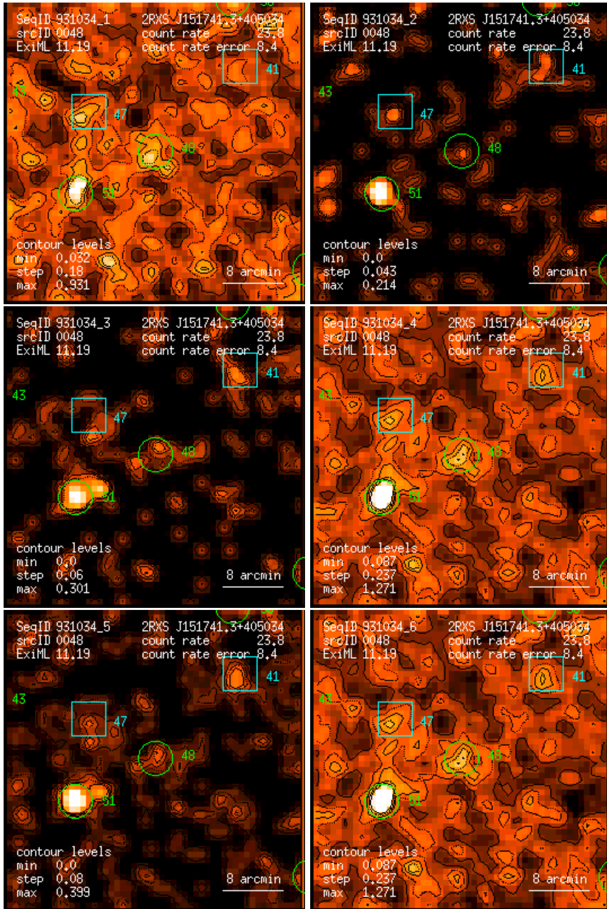
Figure 48: RASS 931034: detection 0048: band rate images, Gaussian filter: (1) PSPC channels 11 – 41, (2) 52 – 90, (3) 91 – 201, (4) 11 – 235, (5) 52 – 201, (6) 11 – 201. Broad band rates in counts/ks. Band rate contour levels in counts/ks/arcmin 2 .
