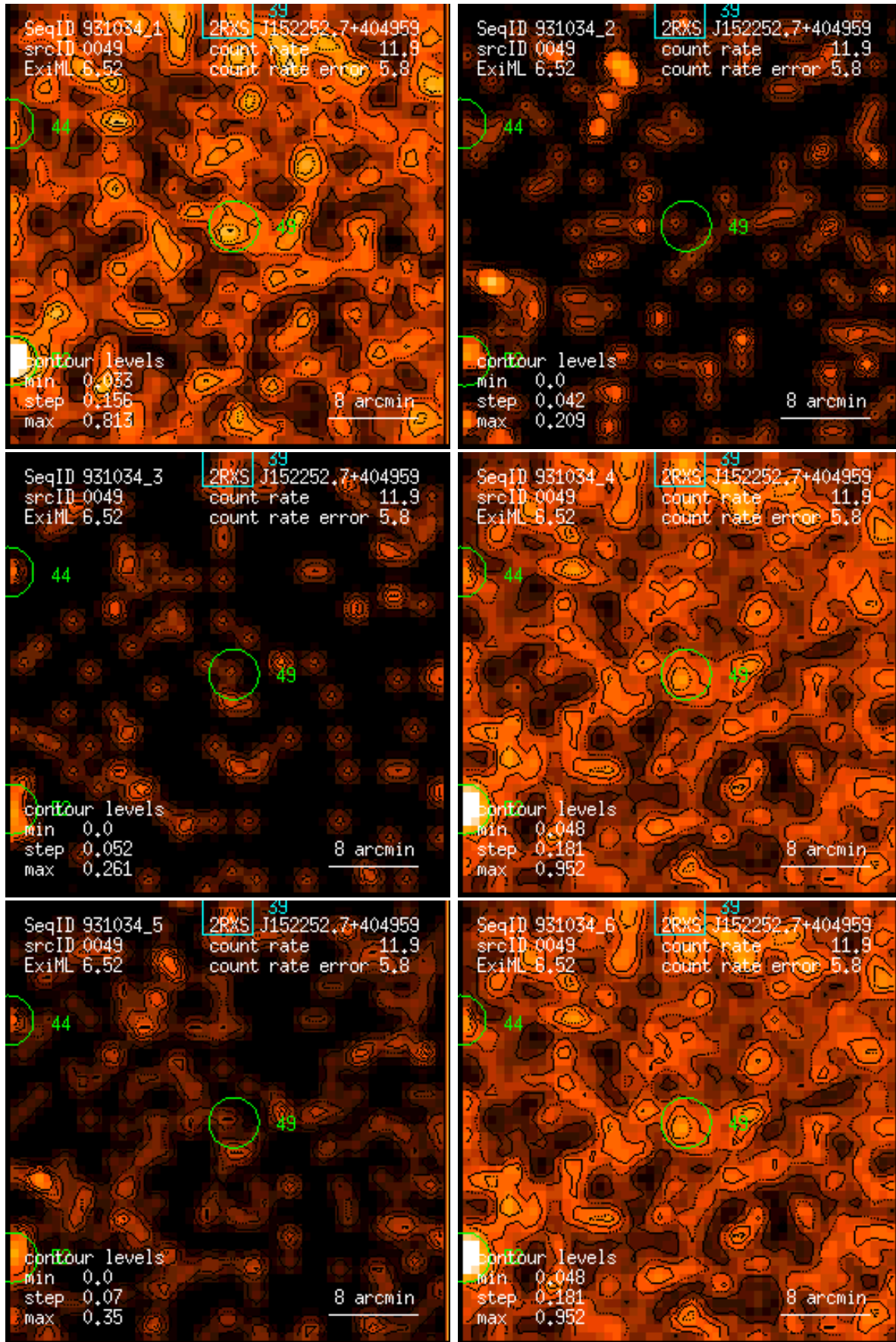
Figure 49: RASS 931034: detection 0049: band rate images, Gaussian filter: (1) PSPC channels 11 – 41, (2) 52 – 90, (3) 91 – 201, (4) 11 – 235, (5) 52 – 201, (6) 11 – 201. Broad band rates in counts/ks. Band rate contour levels in counts/ks/arcmin 2 .
